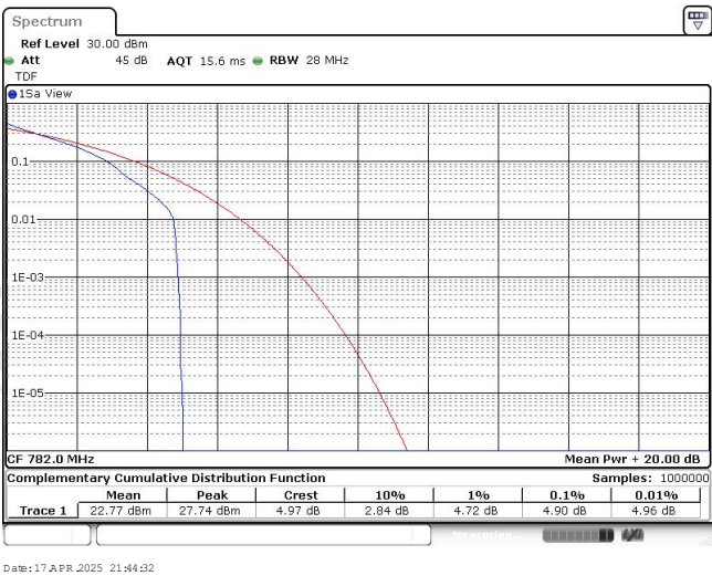
Band13-5MHz-QPSK-23230-1RB#0
