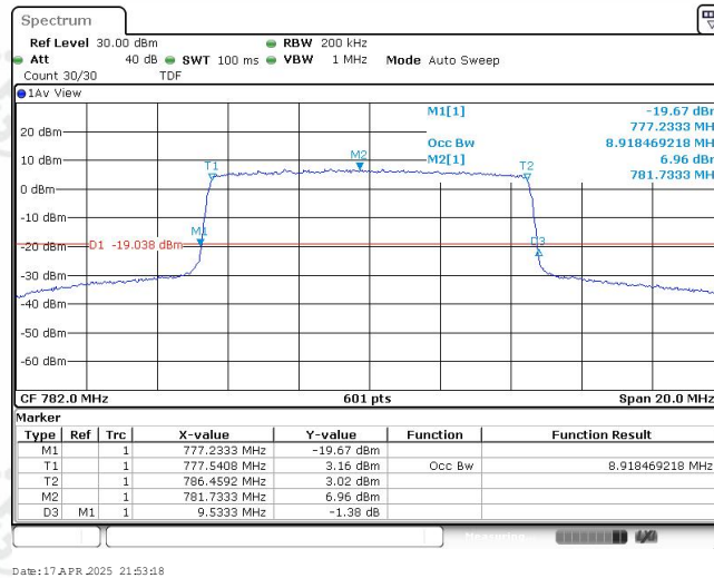
Band13-10MHz-QPSK-23230-50RB#0-8.918
