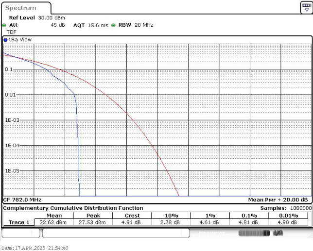
Band13-10MHz-QPSK-23230-1RB#0
