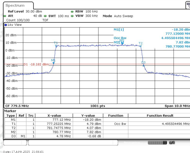
Band13-5MHz-16QAM-23205-25RB#0-4.496
