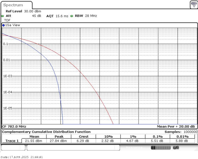
Band13-5MHz-QPSK-23230-25RB#0
