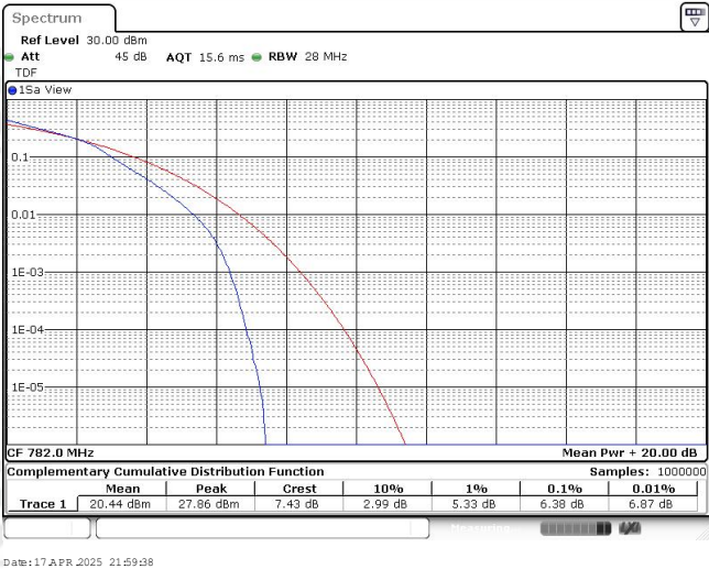
Band13-5MHz-16QAM-23230-25RB#0
