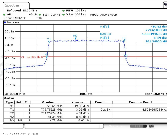
Band13-5MHz-16QAM-23230-25RB#0-4.505
