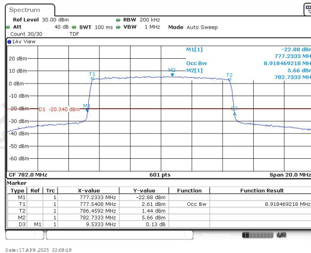
Band13-10MHz-16QAM-23230-50RB#0-8.918
