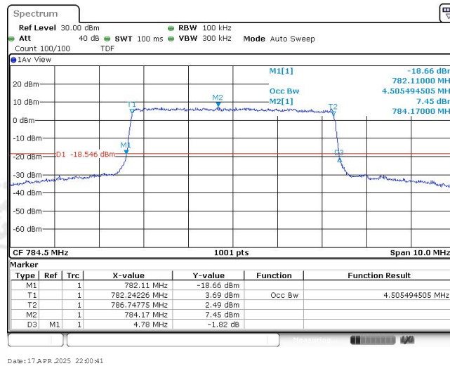
Band13-5MHz-16QAM-23255-25RB#0-4.505
