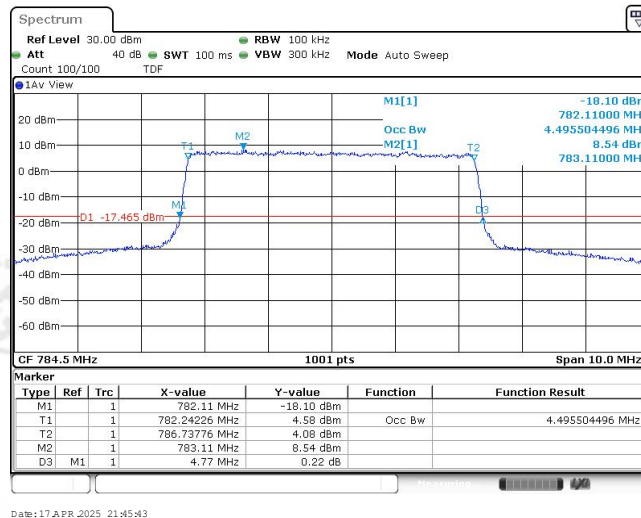
Band13-5MHz-QPSK-23255-25RB#0-4.496
