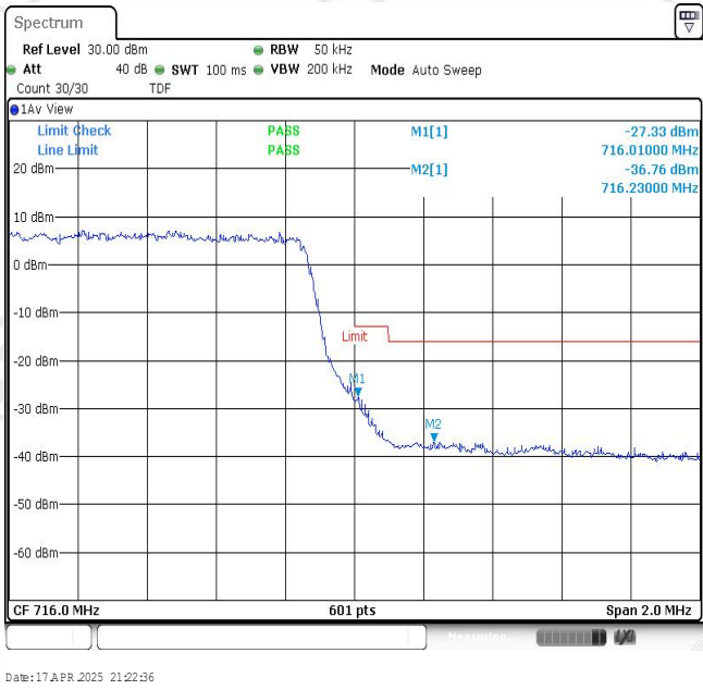
Band12-3MHz-16QAM-23165-15RB#0
