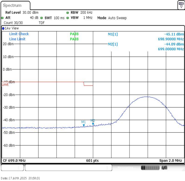
Band12-10MHz-QPSK-23060-1RB#49
