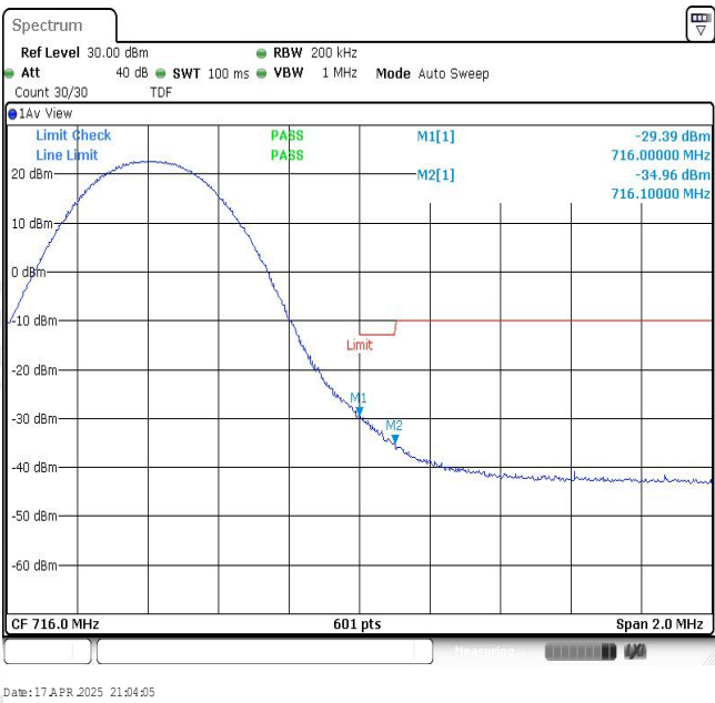
Band12-10MHz-QPSK-23130-1RB#49
