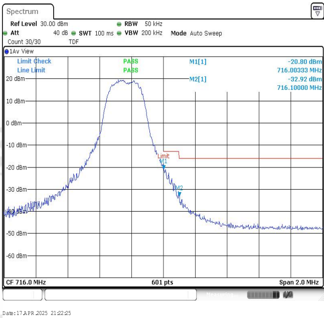
Band12-3MHz-16QAM-23165-1RB#14
