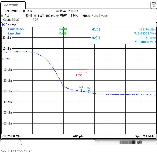
Band12-10MHz-QPSK-23130-50RB#0
