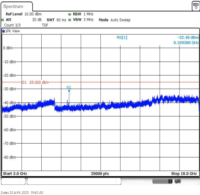
Band7-5MHz-16QAM-21100-1RB#0-Range3:3000~18000MHz
