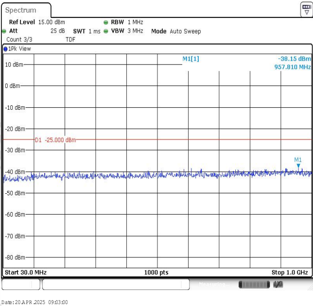
Band7-5MHz-QPSK-21425-1RB#0-Range1:30~1000MHz
