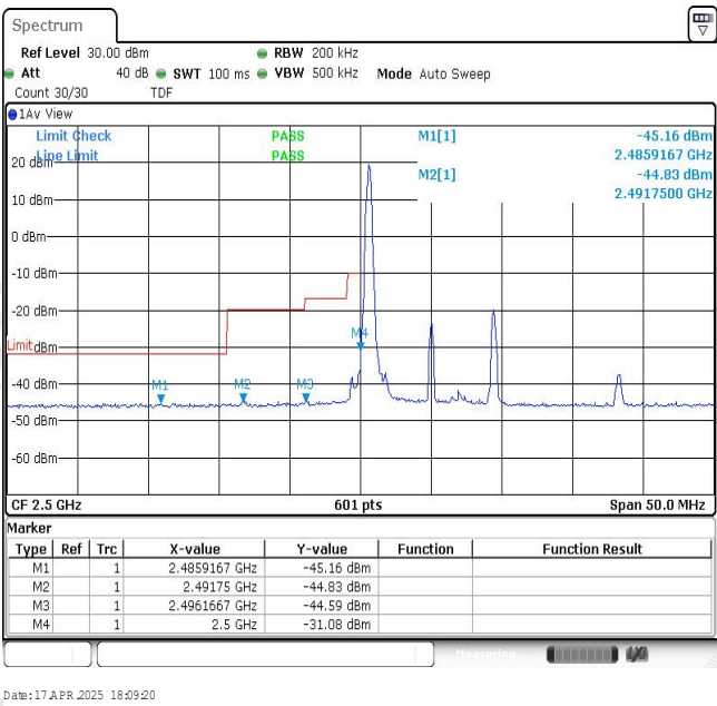
Band7-10MHz-16QAM-20800-1RB#0
