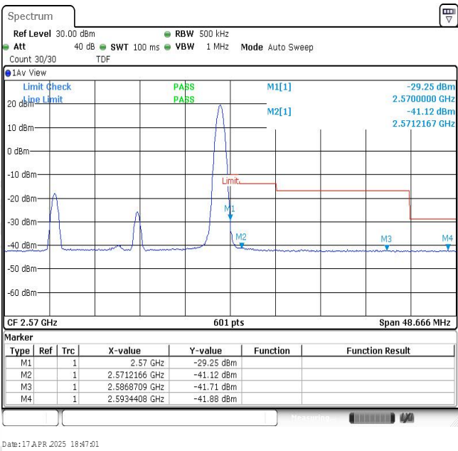
Band7-20MHz-QPSK-21350-1RB#99
