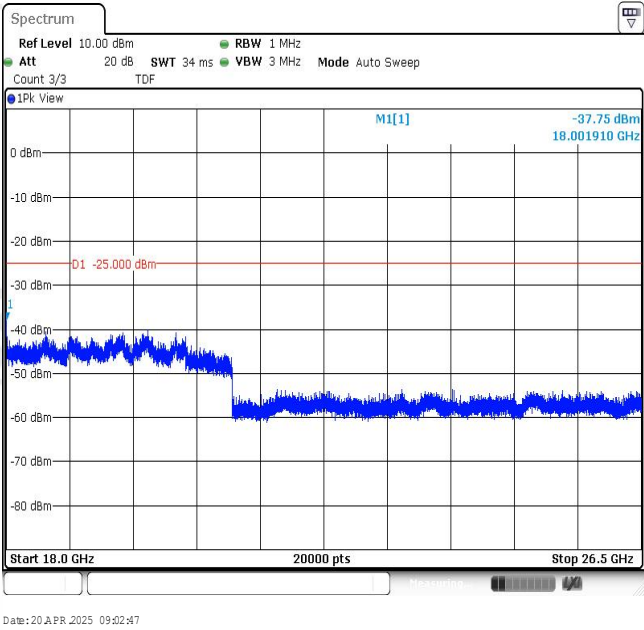
Band7-5MHz-16QAM-21100-1RB#0-Range4:18000~26500MHz
