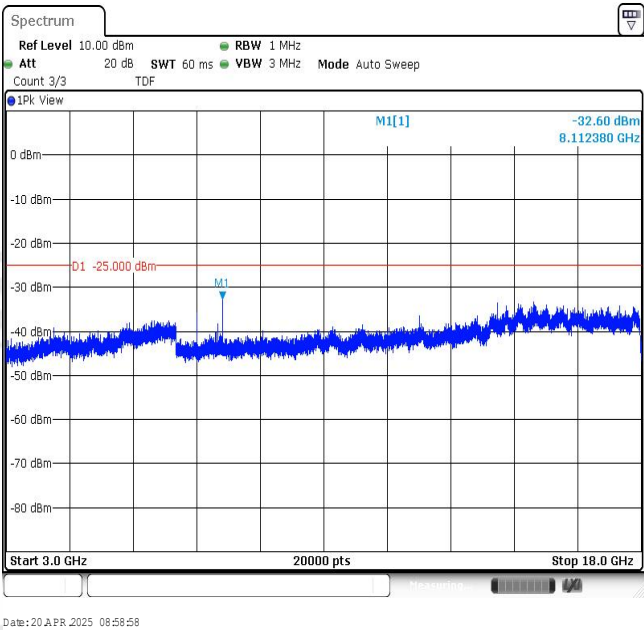
Band7-5MHz-QPSK-20775-1RB#0-Range3:3000~18000MHz
