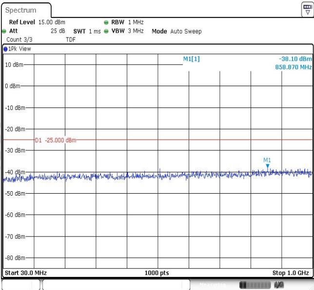
Band7-5MHz-16QAM-21425-1RB#0-Range1:30~1000MHz
