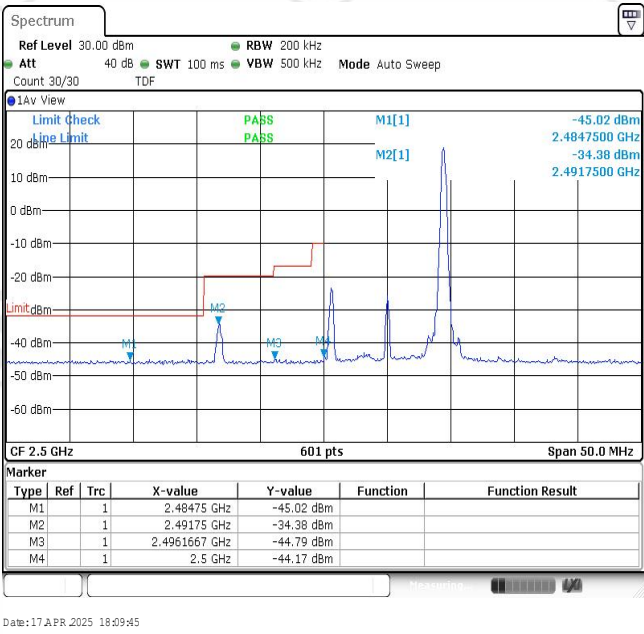
Band7-10MHz-16QAM-20800-1RB#49
