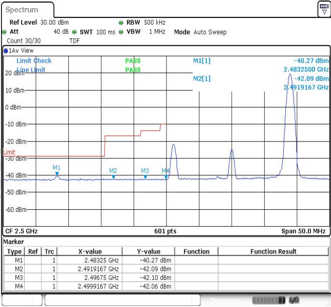
Band7-20MHz-QPSK-20850-1RB#0
