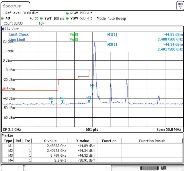
Band7-10MHz-QPSK-20800-1RB#0
