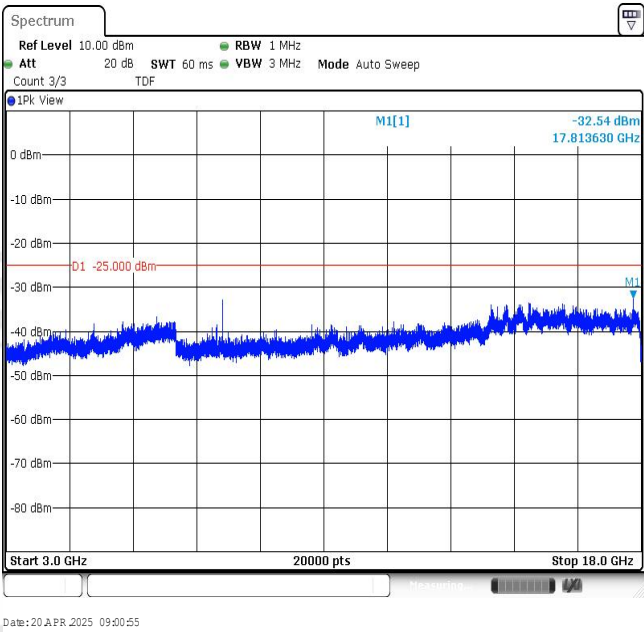
Band7-5MHz-QPSK-21100-1RB#0-Range3:3000~18000MHz
