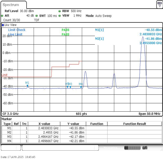
Band7-20MHz-16QAM-20850-1RB#99
