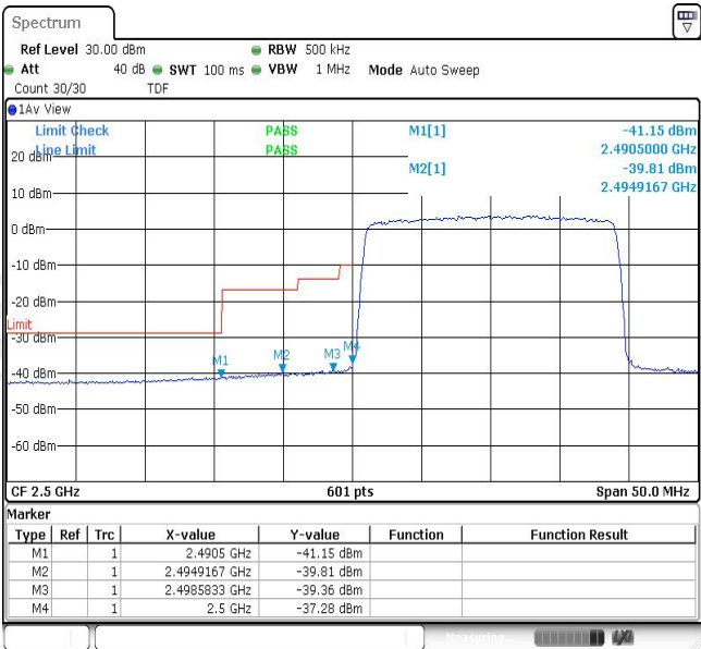
Band7-20MHz-16QAM-20850-100RB#0
