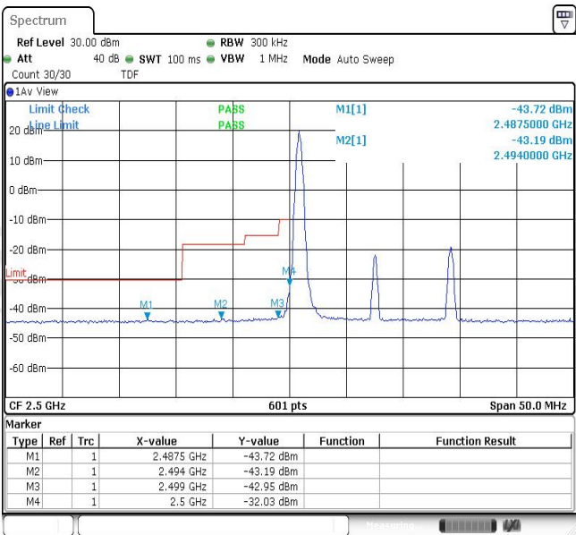
Band7-15MHz-16QAM-20825-1RB#0
