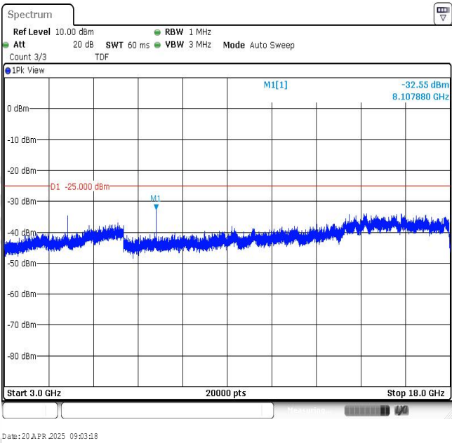
Band7-5MHz-QPSK-21425-1RB#0-Range3:3000~18000MHz
