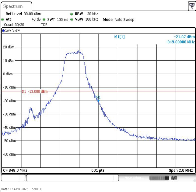
Band5-1.4MHz-QPSK-20643-1RB#5
