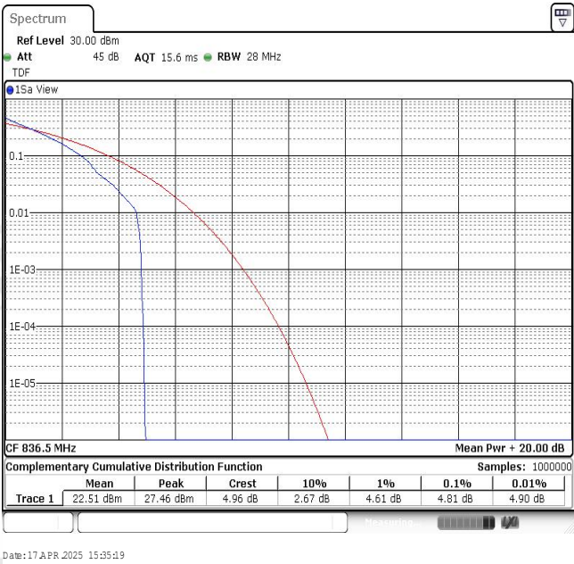
Band5-10MHz-QPSK-20525-1RB#0
