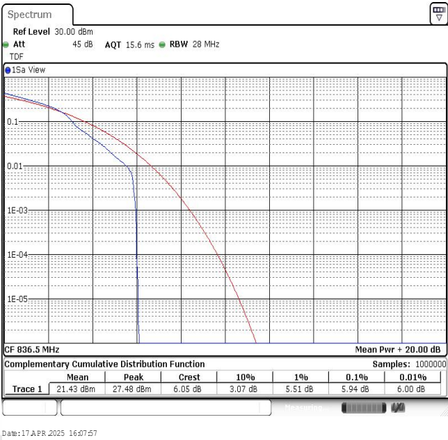
Band5-10MHz-16QAM-20525-1RB#0
