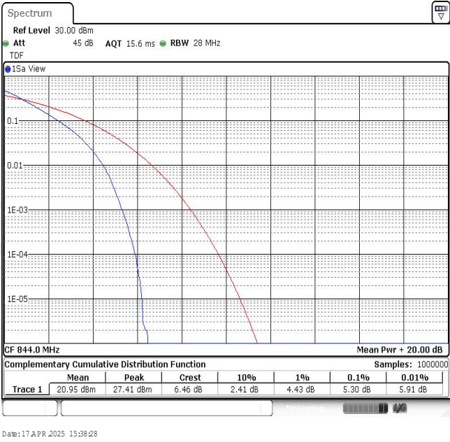
Band5-10MHz-QPSK-20600-50RB#0
