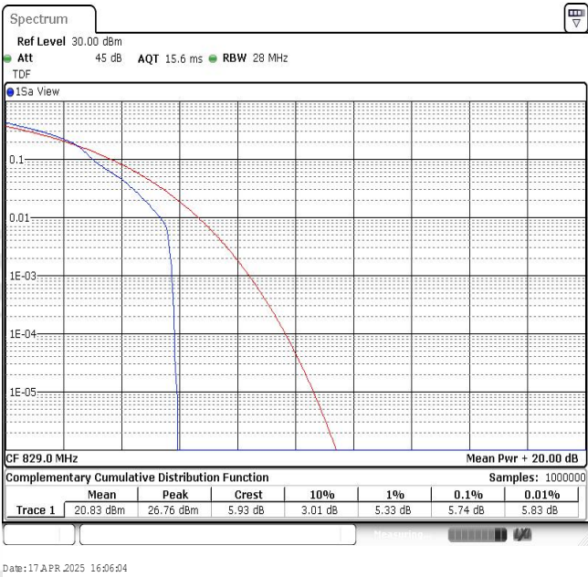
Band5-10MHz-16QAM-20450-1RB#0
