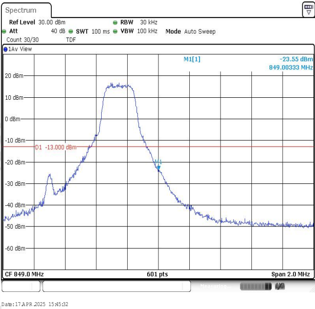
Band5-1.4MHz-16QAM-20643-1RB#5
