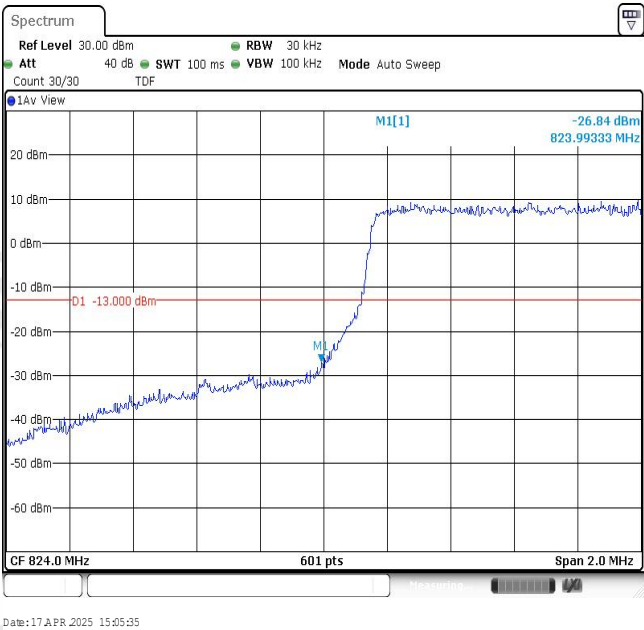
Band5-1.4MHz-QPSK-20407-6RB#0
