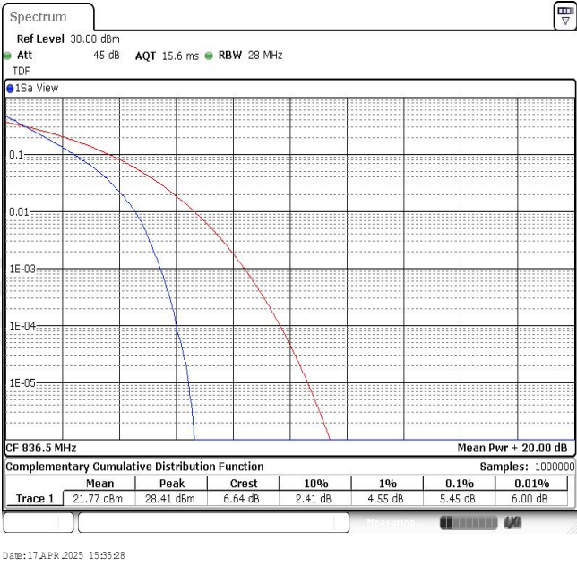
Band5-10MHz-QPSK-20525-50RB#0
