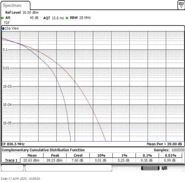
Band5-10MHz-16QAM-20525-50RB#0
