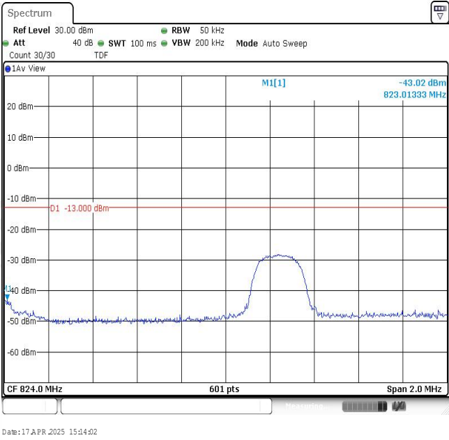
Band5-3MHz-QPSK-20415-1RB#14
