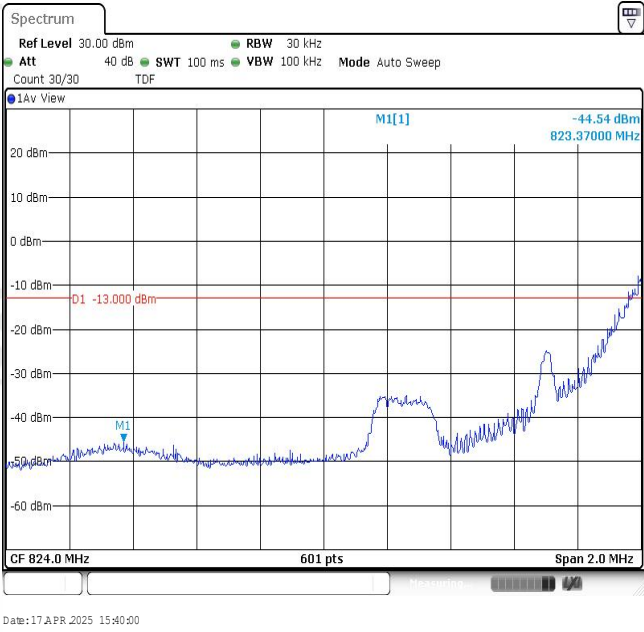
Band5-1.4MHz-16QAM-20407-1RB#5
