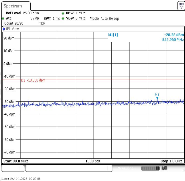
Band2-3MHz-QPSK-18900-1RB#0-Range1:30~1000MHz
