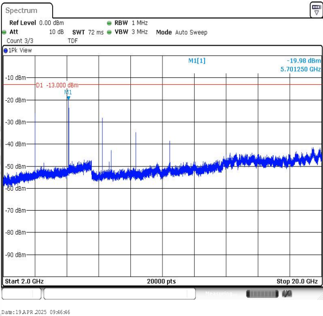
Band2-10MHz-16QAM-19150-1RB#0-Range3:2000~20000MHz
