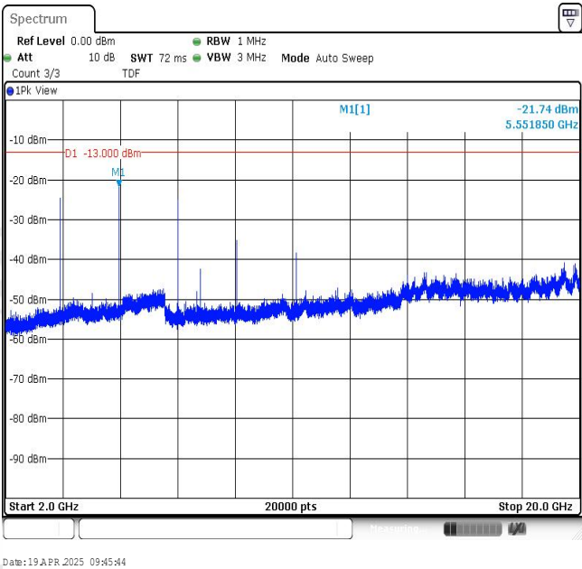
Band2-10MHz-16QAM-18650-1RB#0-Range3:2000~20000MHz
