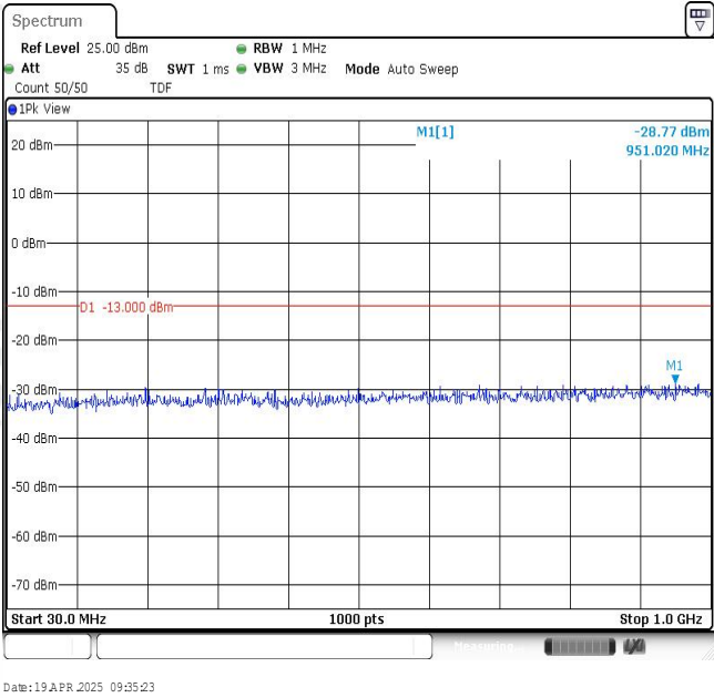
Band2-15MHz-QPSK-18675-1RB#0-Range1:30~1000MHz
