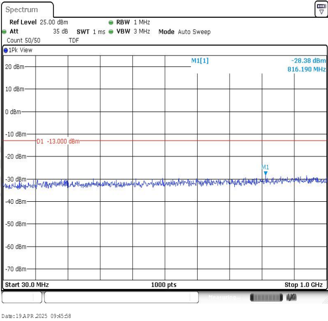
Band2-10MHz-16QAM-18900-1RB#0-Range1:30~1000MHz
