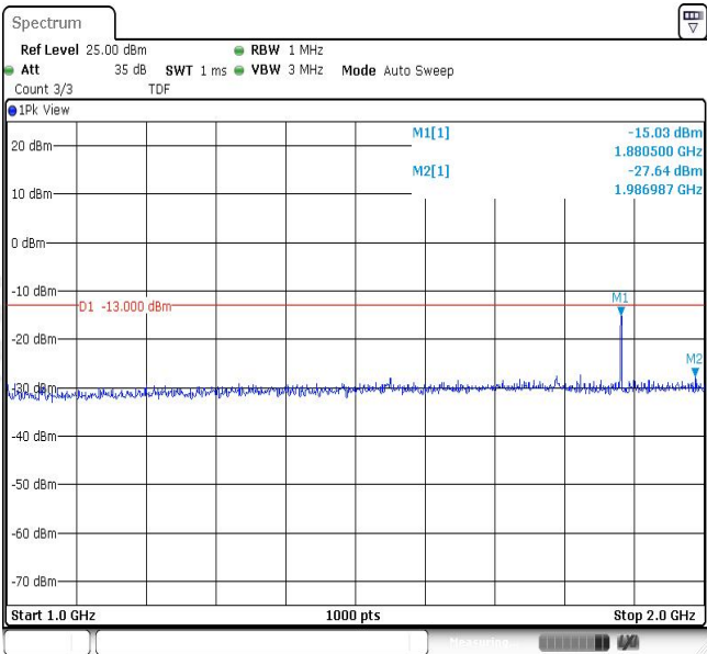
Band2-1.4MHz-16QAM-18900-1RB#0-Range2:1000~2000MHz
