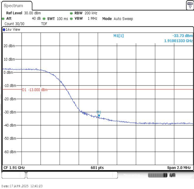
Band2-10MHz-16QAM-19150-50RB#0
