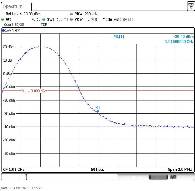
Band2-10MHz-QPSK-19150-1RB#49
