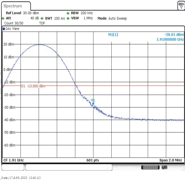
Band2-10MHz-16QAM-19150-1RB#49
