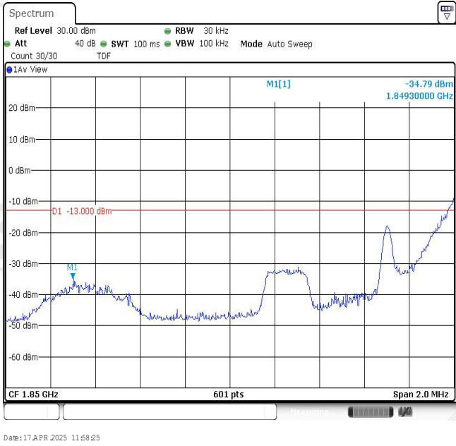
Band2-1.4MHz-16QAM-18607-1RB#5
