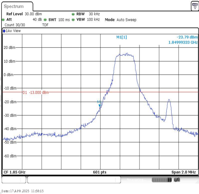
Band2-1.4MHz-16QAM-18607-1RB#0
