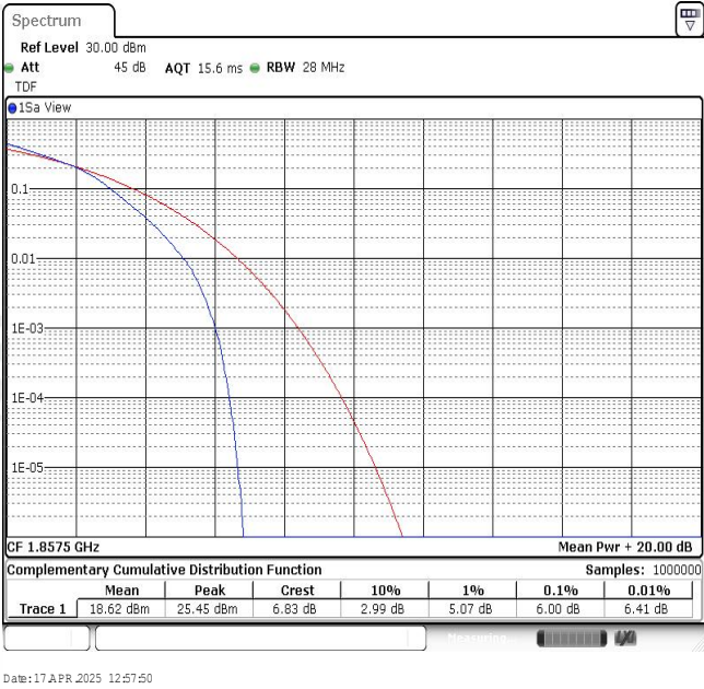
Band2-15MHz-16QAM-18675-75RB#0
