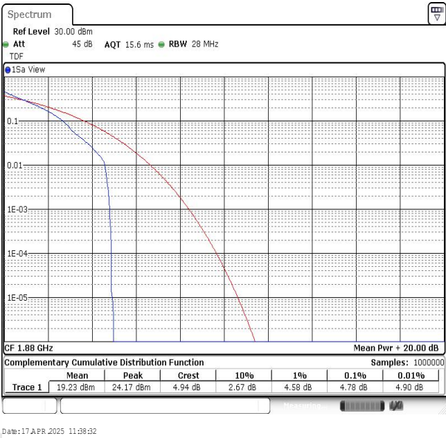
Band2-15MHz-QPSK-18900-1RB#0
