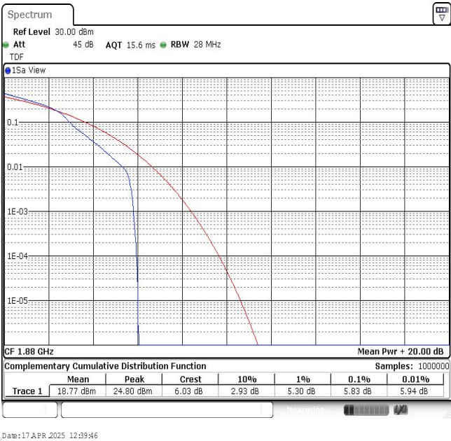
Band2-10MHz-16QAM-18900-1RB#0
