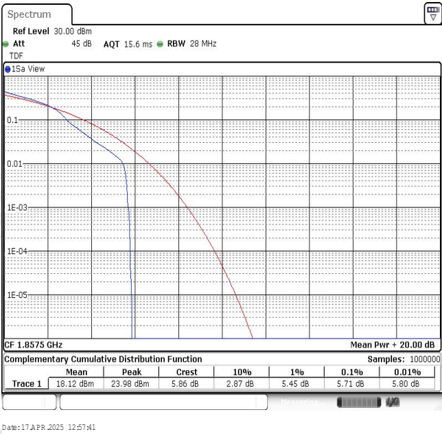
Band2-15MHz-16QAM-18675-1RB#0
