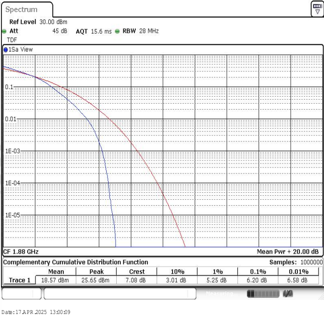
Band2-15MHz-16QAM-18900-75RB#0
