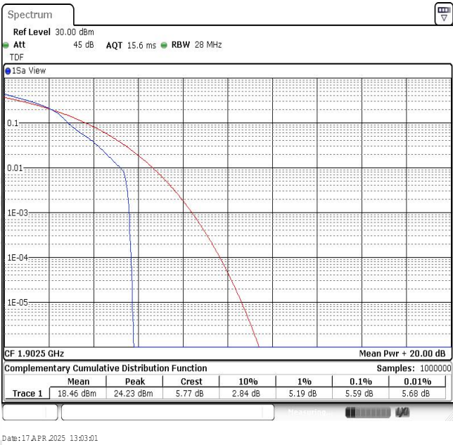
Band2-15MHz-16QAM-19125-1RB#0
