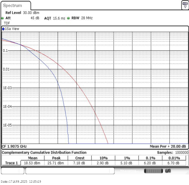
Band2-5MHz-16QAM-19175-25RB#0
