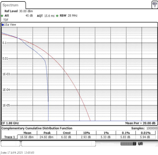
Band2-15MHz-16QAM-18900-1RB#0
