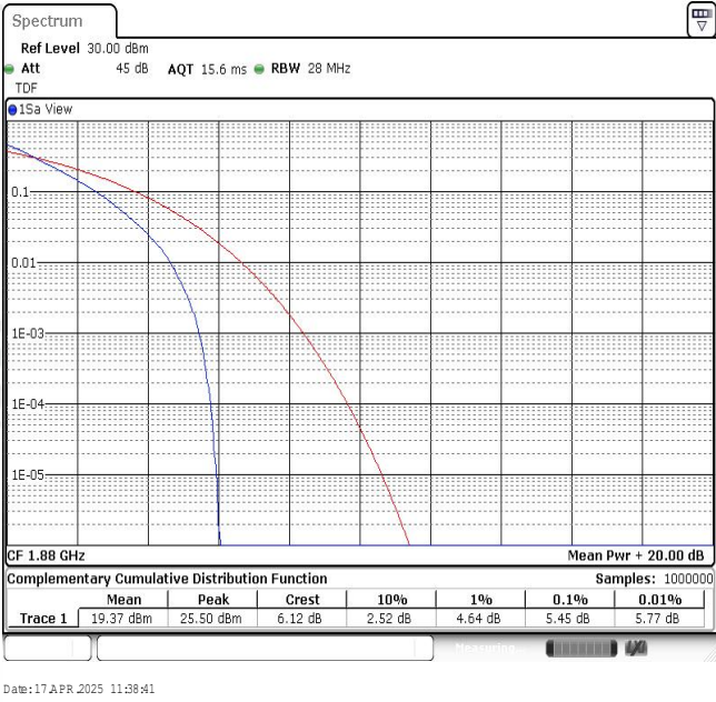
Band2-15MHz-QPSK-18900-75RB#0
