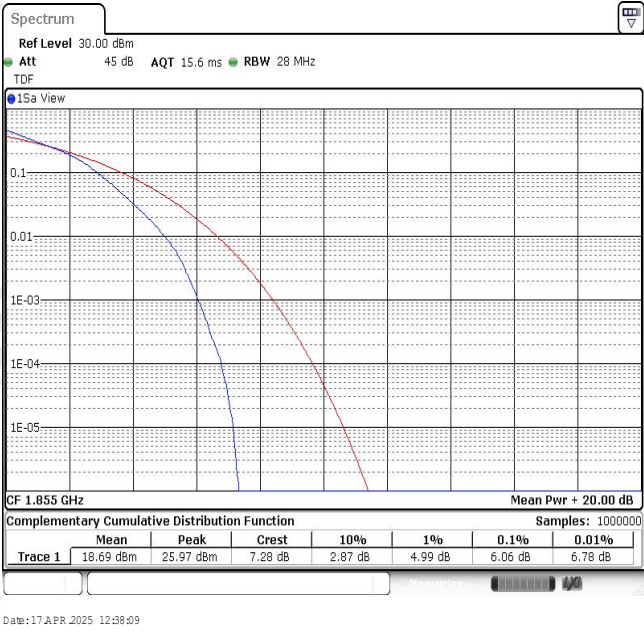
Band2-10MHz-16QAM-18650-50RB#0
