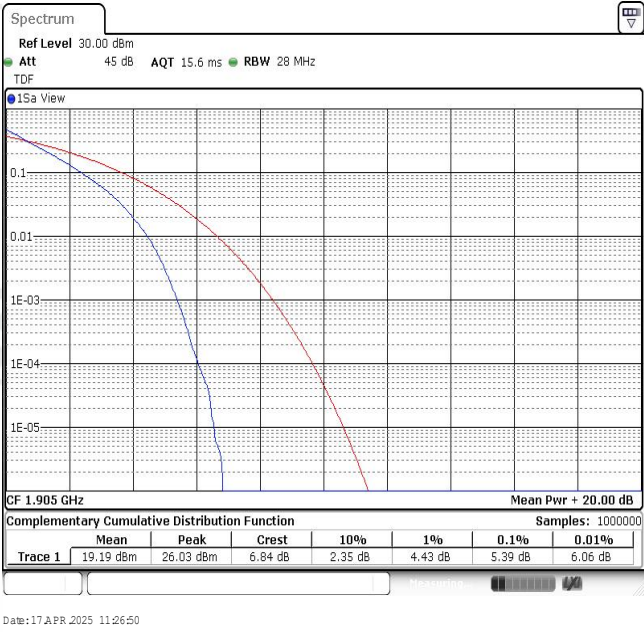
Band2-10MHz-QPSK-19150-50RB#0
