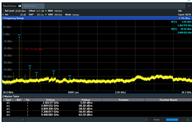
\pi/4 -DQPSK on Channel 00
