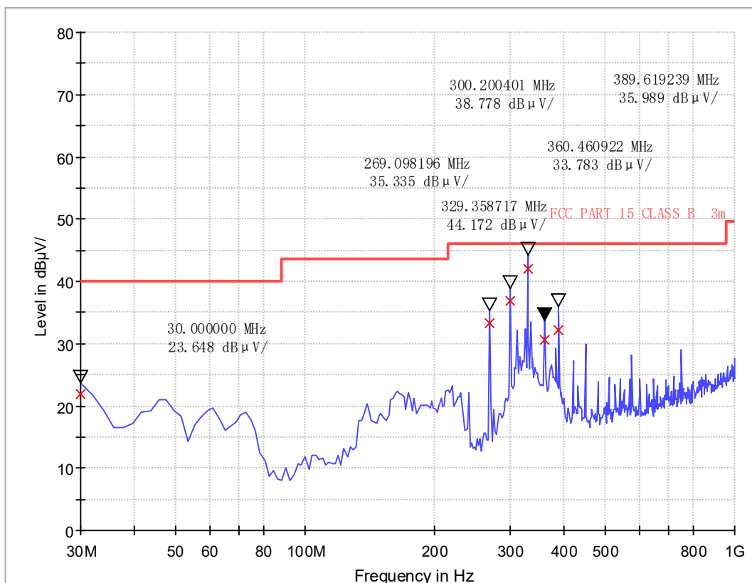
(Plot C: Test Antenna Vertical 30M - 1G)
