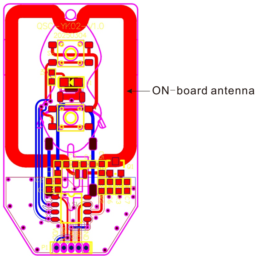
Remote control board frame diagram
