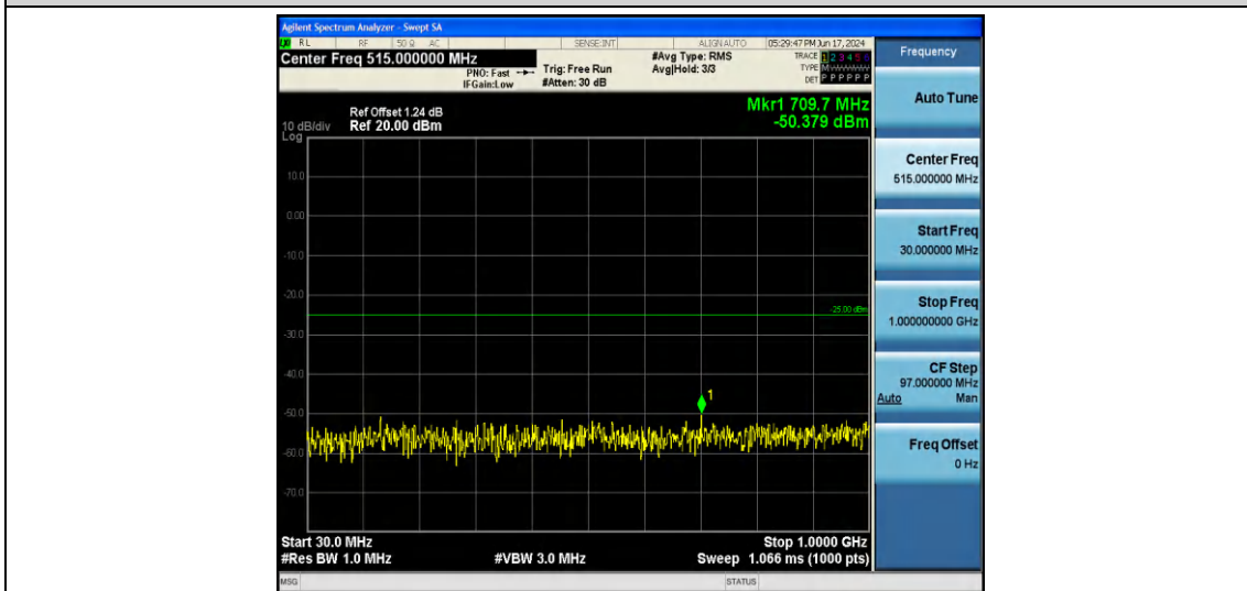
Band41-20MHz-QPSK-40620-1RB#0-Range1:30~1000MHz
