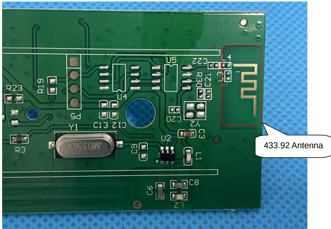
INTERNAL VIEW OF EUT (FIGURE 3)
