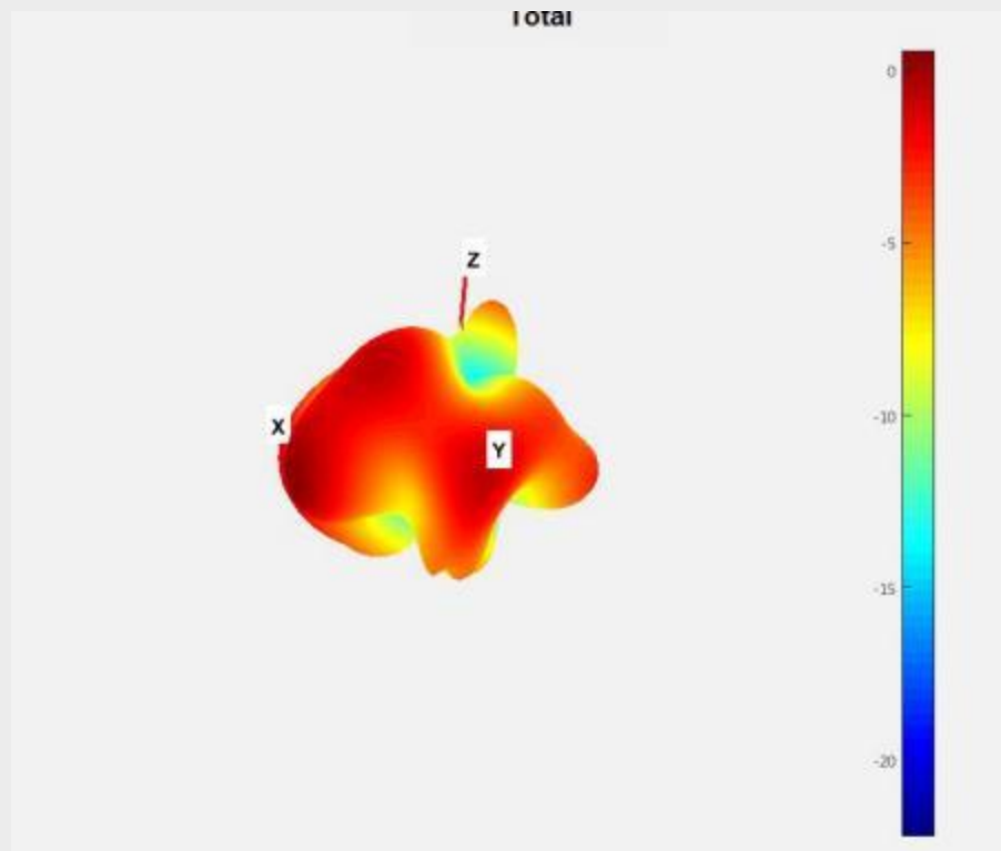
WiFi 5500MHz 3D
