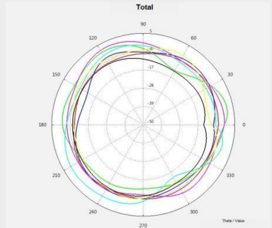
BT 2450MHz 2D
