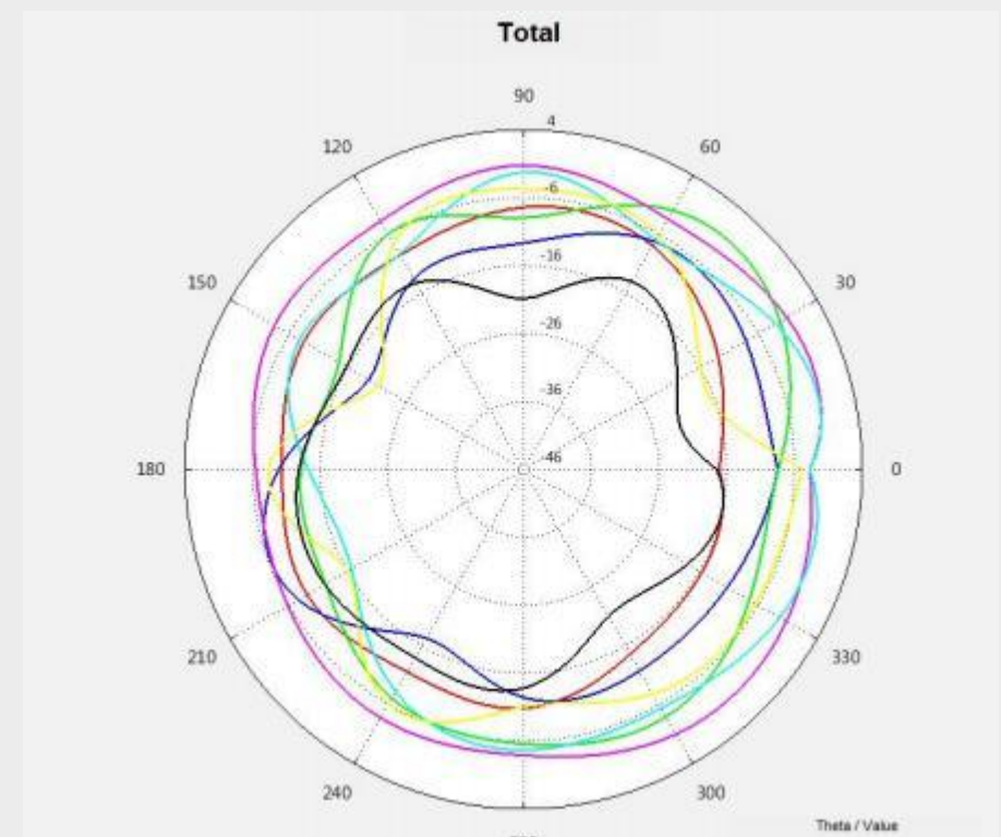
WiFi 5500MHz 2D
