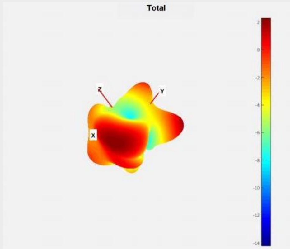
WiFi 2450MHz 3D
