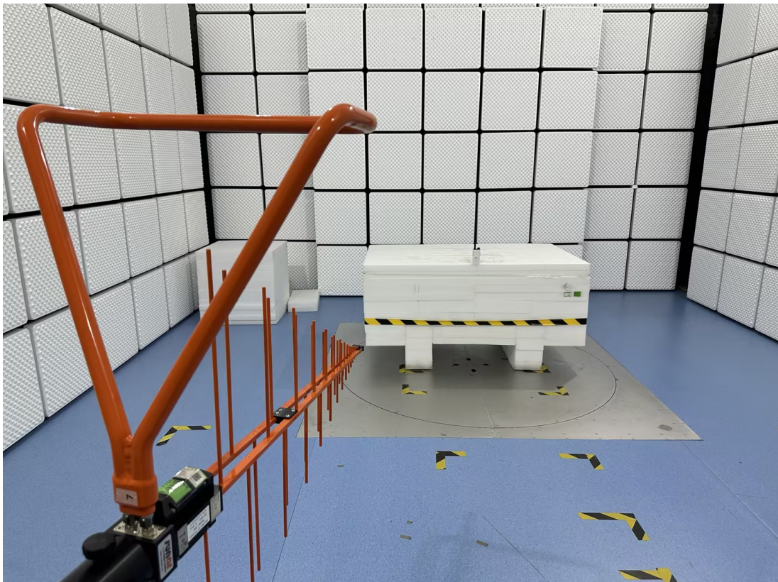
RSE-Back View(Below 1GHz)
