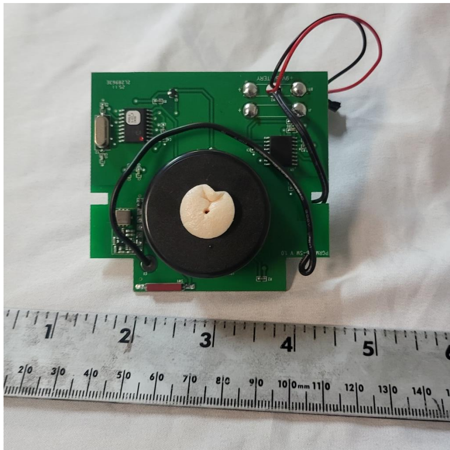
Figure 3. PCBA Bottom
