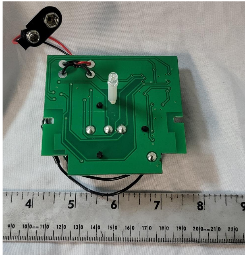
Figure 2. Top of PCBA
