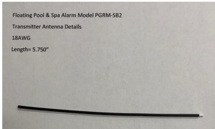
Figure 4. Antenna details
