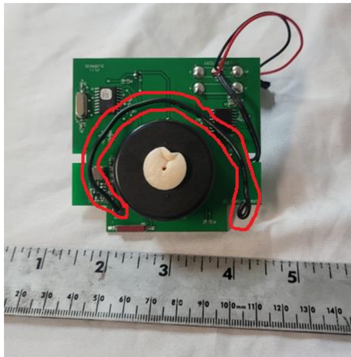
Figure 5. Antenna location and placement
