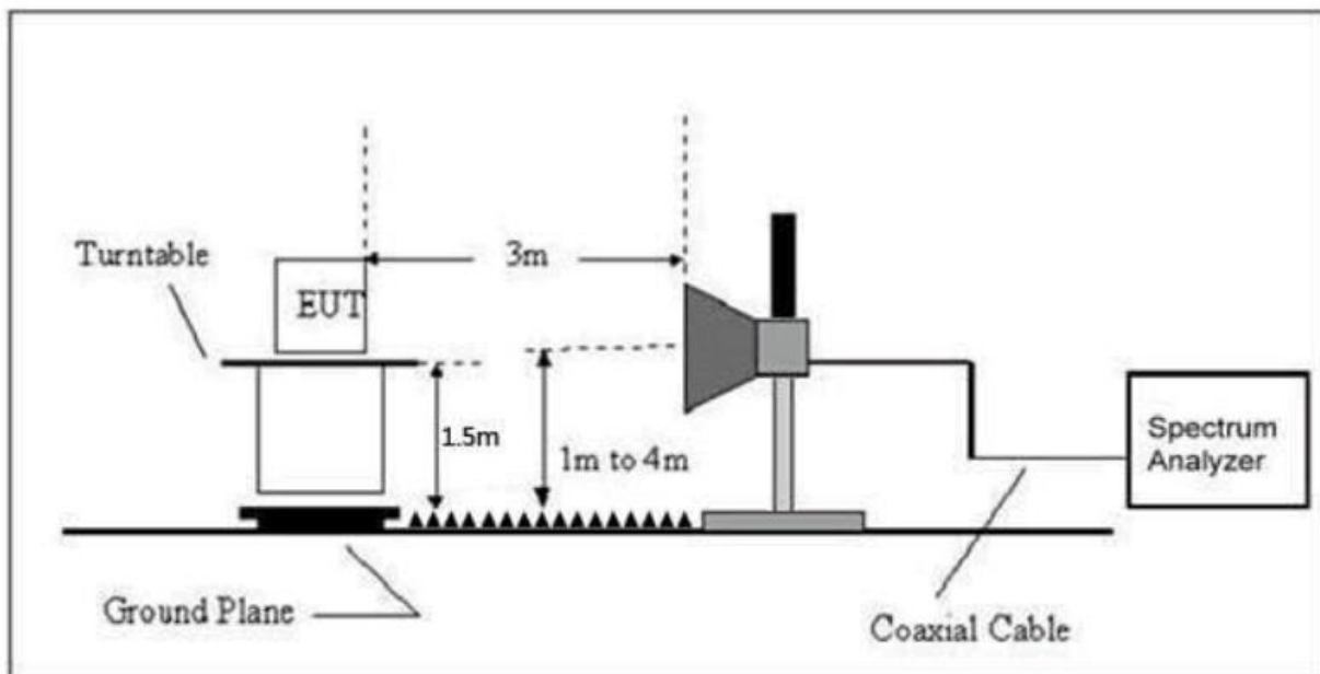
Figure 4. Radiated Emissions above 1 GHz
