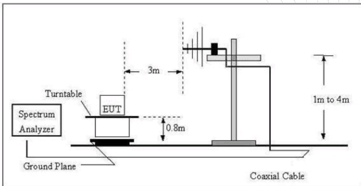
Figure 3. Radiated Emissions 30 MHz to 1 GHz
