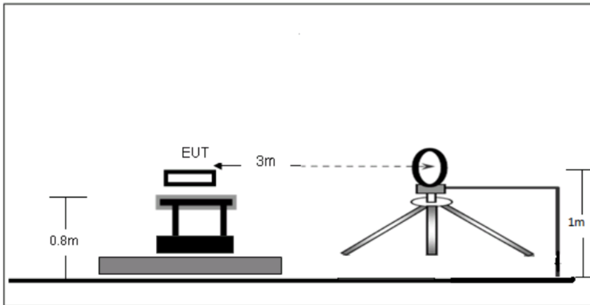
Figure 2. Radiated Emissions Below 30 MHz
