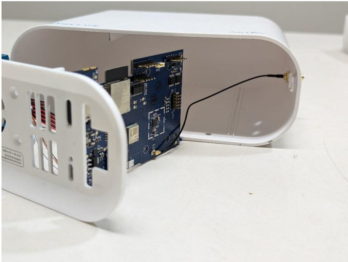
Photograph 4 – View of the PCB Mounting in the Enclosure with connection to Antenna Port
