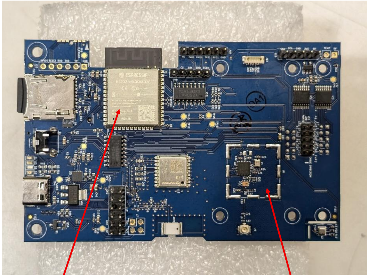
Photograph 1 – Front View of the PCBA
