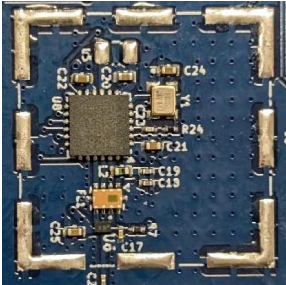
Photograph 3 – Closeup of RF Circuitry
