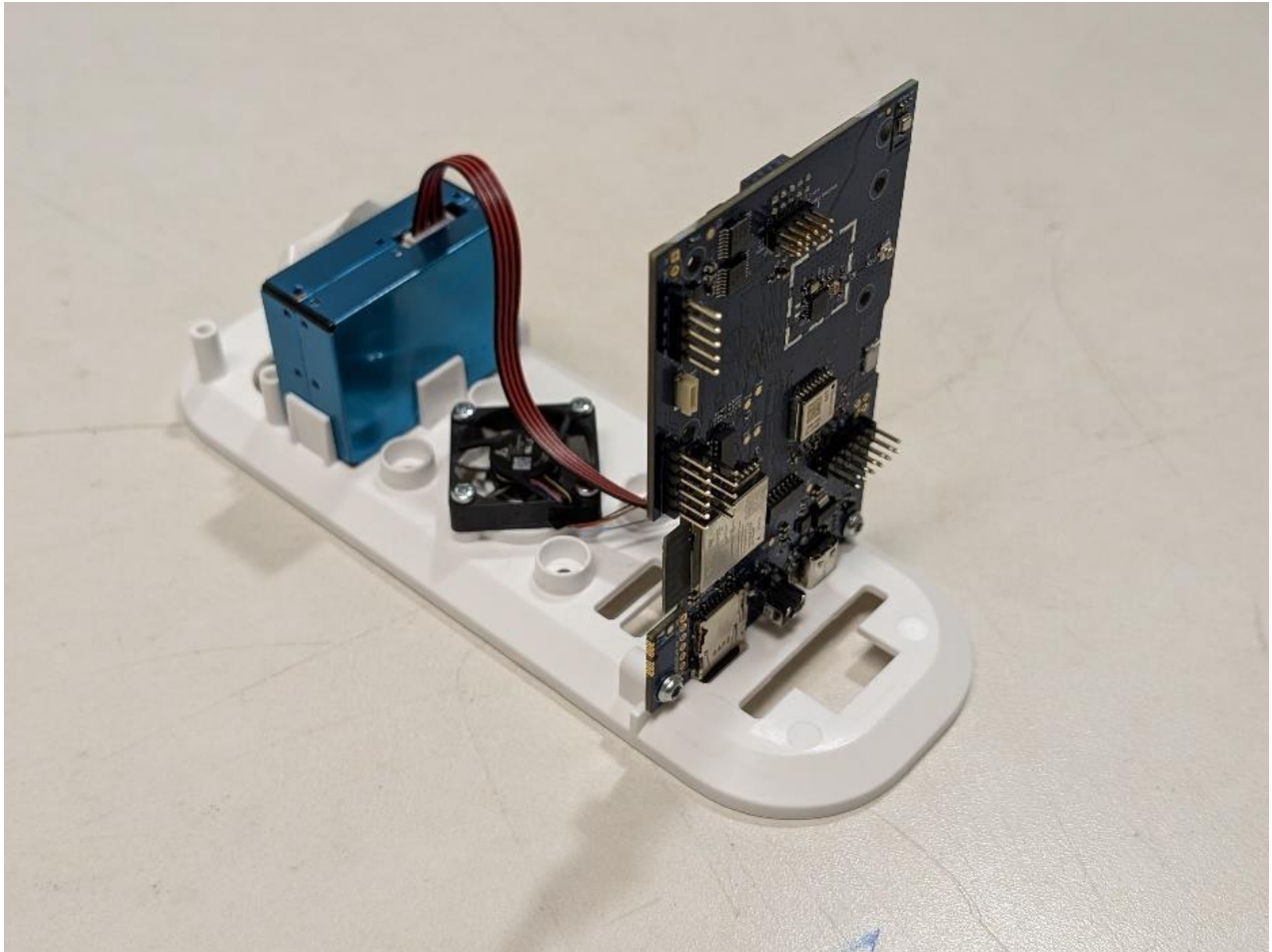
Photograph 5 – View of the PCB removed from enclosure housing
