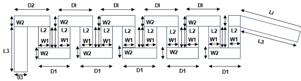
Antenna Dimensions
