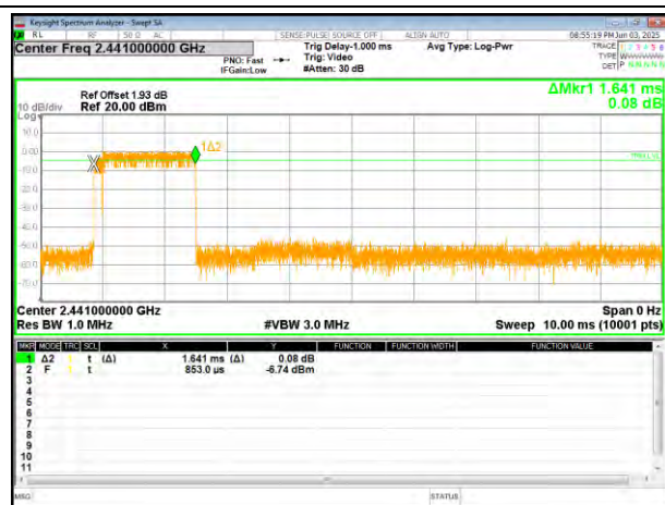
3DH5-2441MHz-One burst
