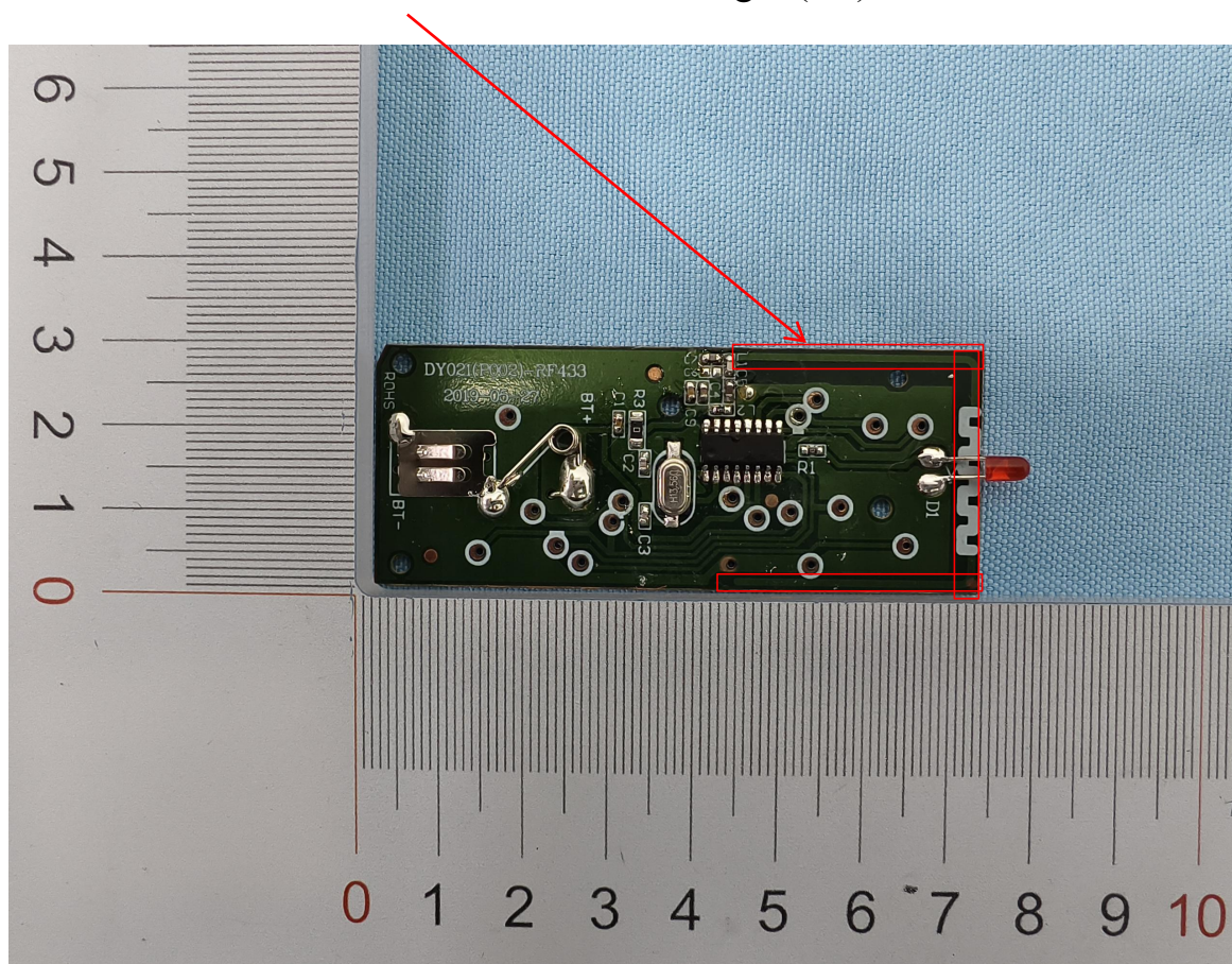
Antenna Photo &amp; Length (cm)
