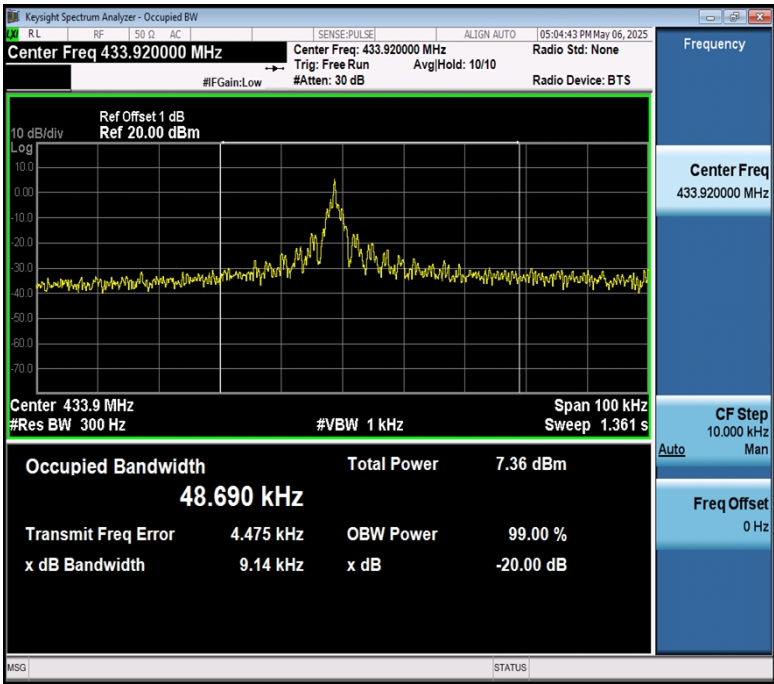
20dB Bandwidth
