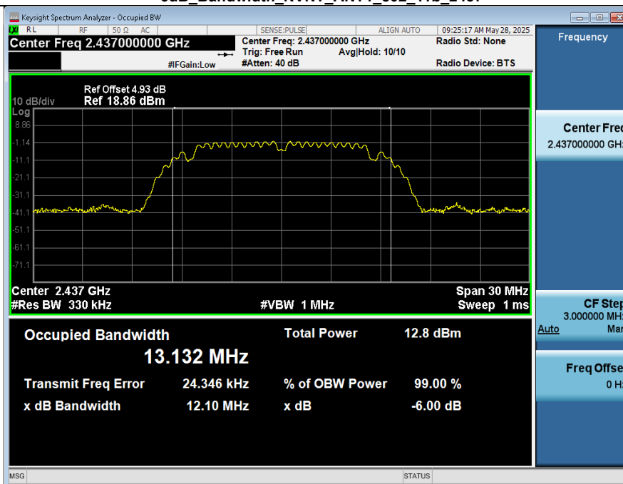
-6dB Bandwidth_NVNT_ANT1_802_11b_2437
