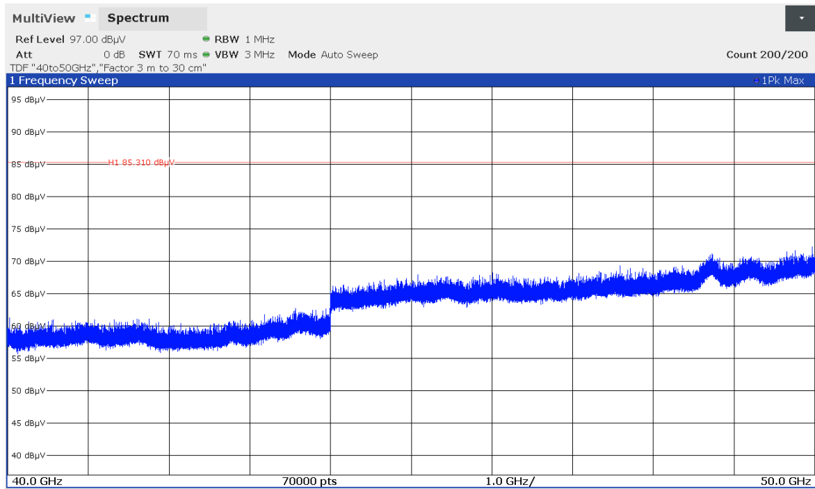
Figure 7.6-13: Radiated spurious emissions 40-50 GHz Low Ch
