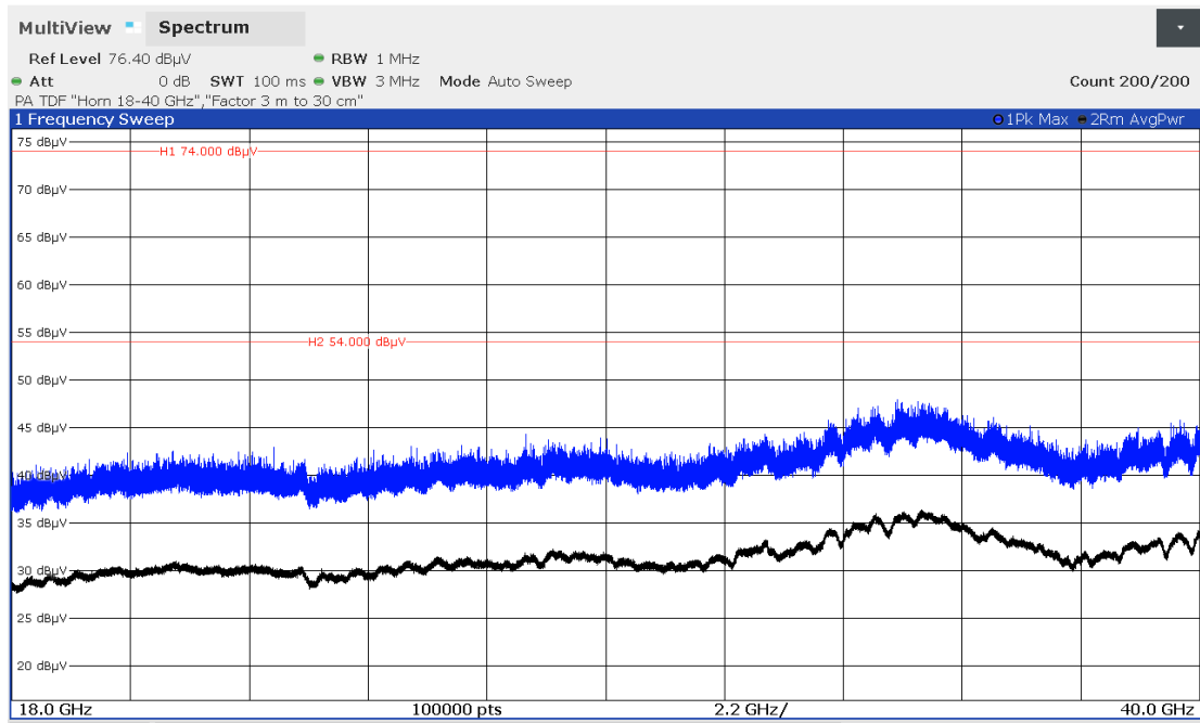
Figure 7.6-3: Radiated spurious emissions 18-40 GHz High Ch
