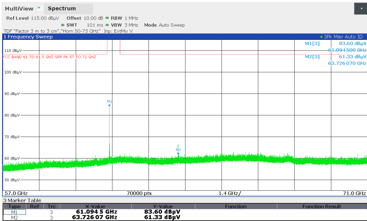
Figure 7.6-15: Radiated spurious emissions 50-75 GHz mask Low Ch
