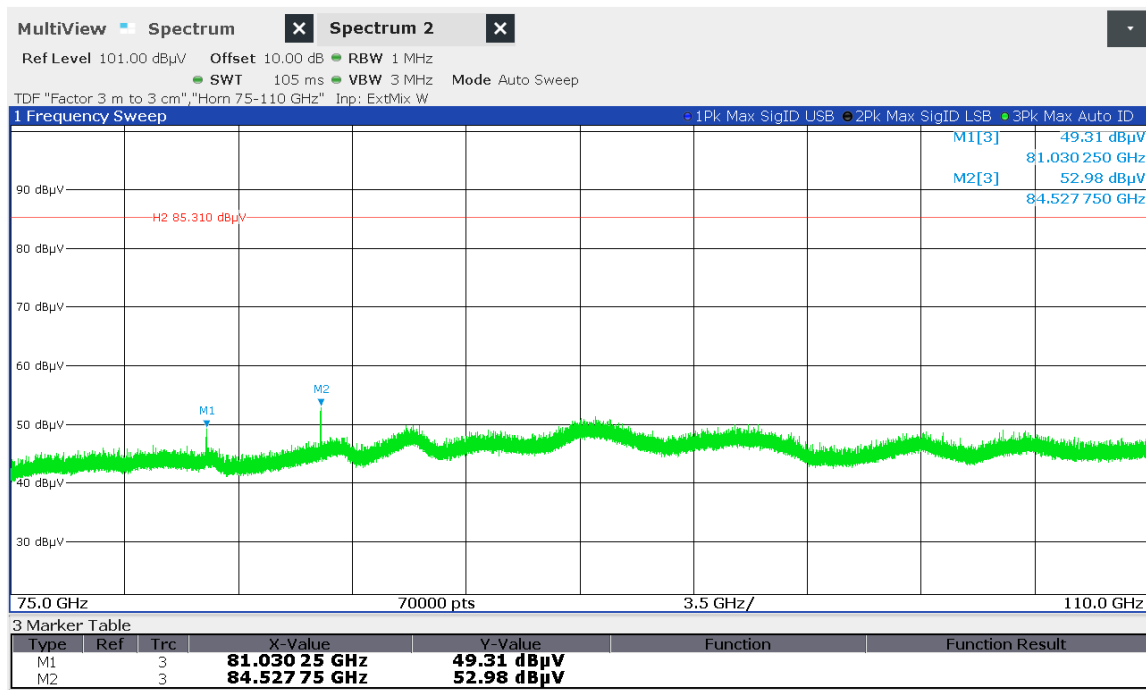
Figure 7.6-16: Radiated spurious emissions 75 GHz-110 GHz Low Ch
