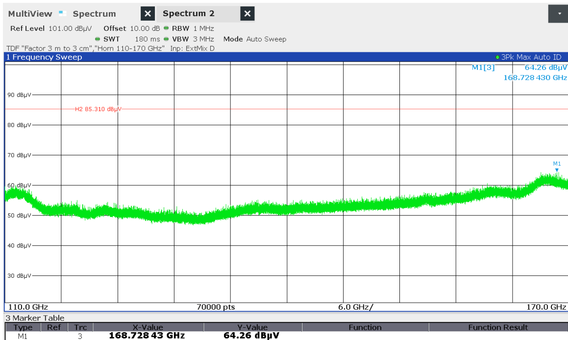
Figure 7.6-8: Radiated spurious emissions 110-170 GHz High Ch
