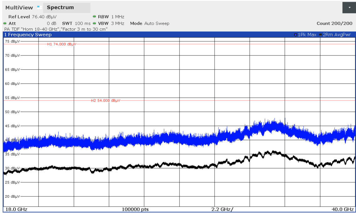
Figure 7.6-12: Radiated spurious emissions 18-40 GHz Low Ch
