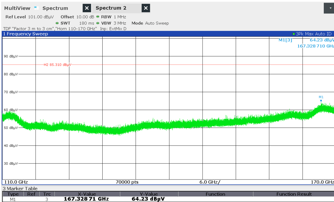
Figure 7.6-17: Radiated spurious emissions 110-170 GHz Low Ch
