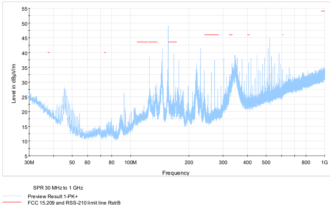
Figure 7.6-10: Radiated spurious emissions below 1000 MHz Low Ch
