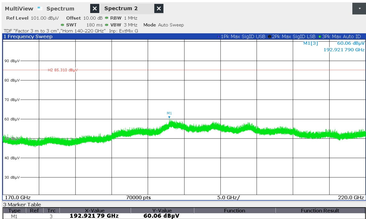
Figure 7.6-19: Radiated spurious emissions 170-220 GHz Low Ch
