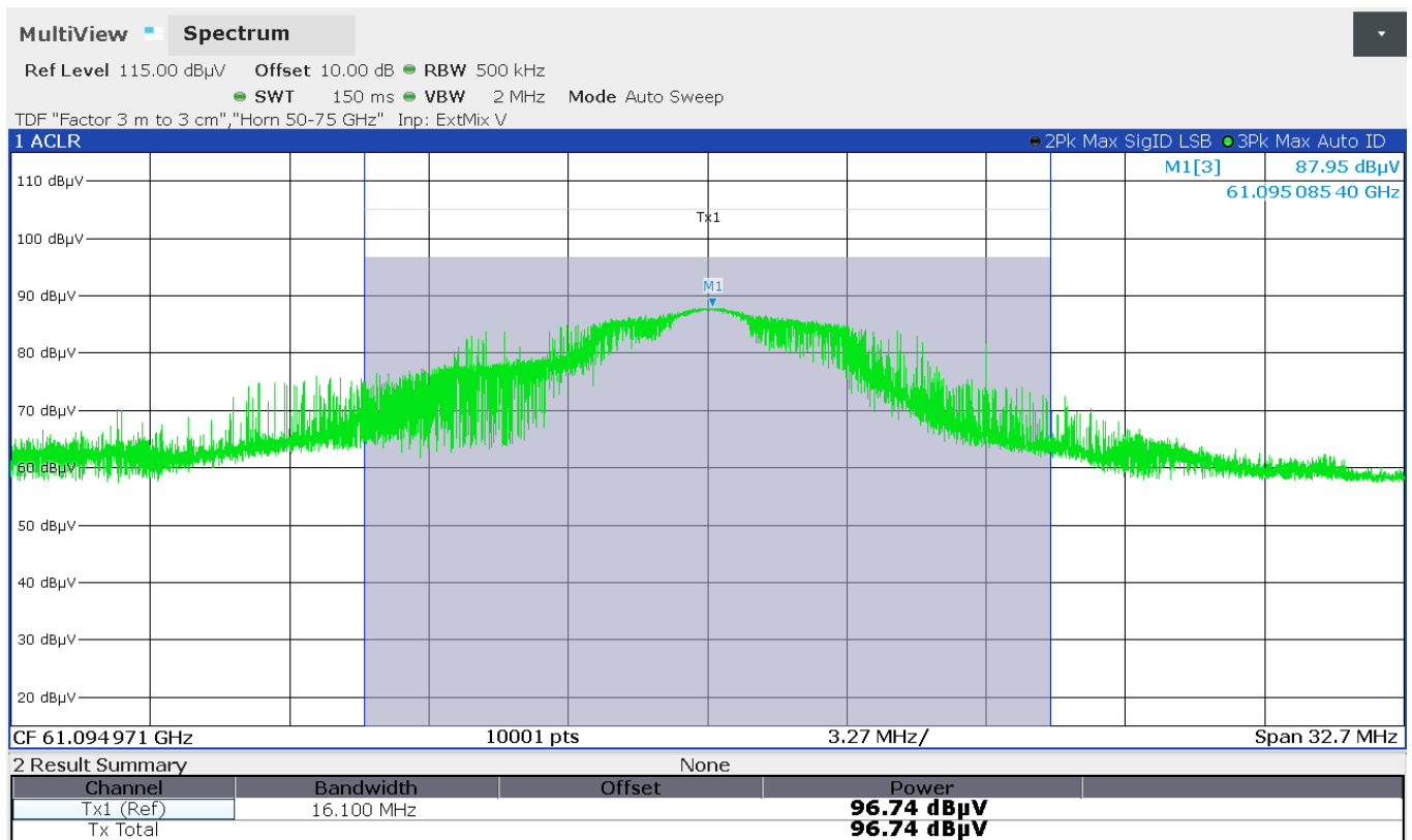
Figure 7.5-2: Field strength of fundamental - Low Ch
