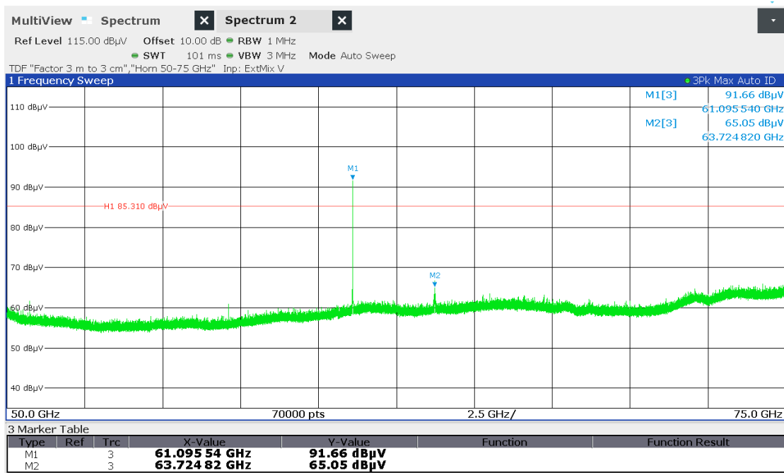
Figure 7.6-14: Radiated spurious emissions 50-75 GHz Low Ch
