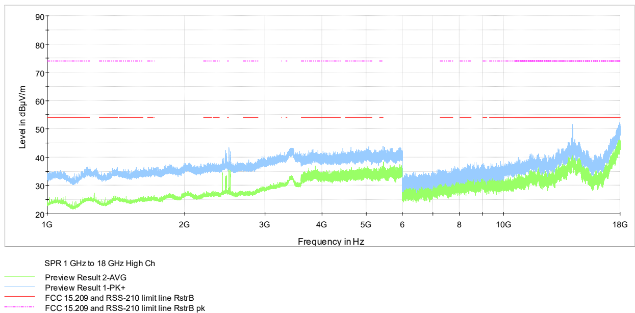
Figure 7.6-2: Radiated spurious emissions above 1-18 GHz High Ch
