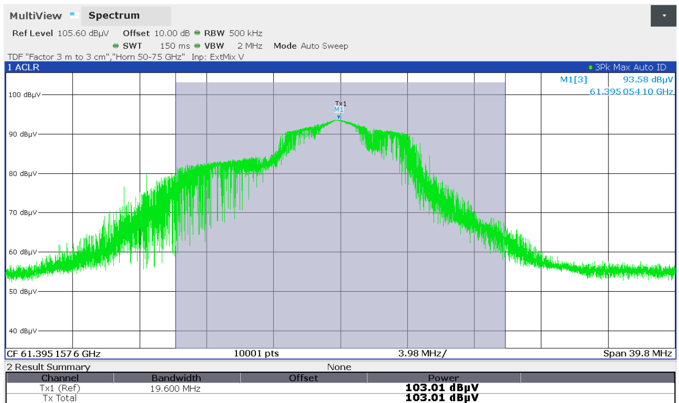
Figure 7.5-1: Field strength of fundamental - High Ch
