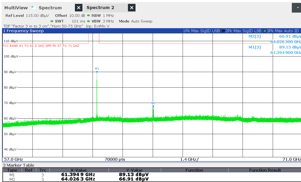
Figure 7.6-6: Radiated spurious emissions 50-75 GHz Mask High Ch
