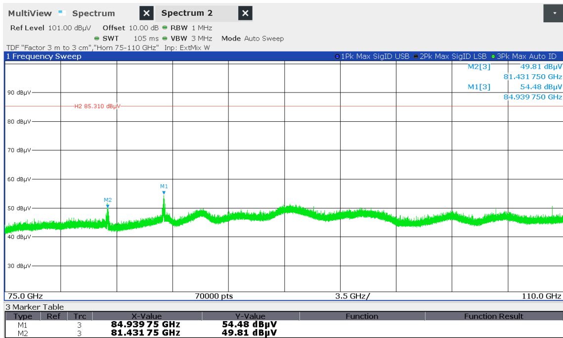
Figure 7.6-7: Radiated spurious emissions 75 GHz-110 GHz High Ch
