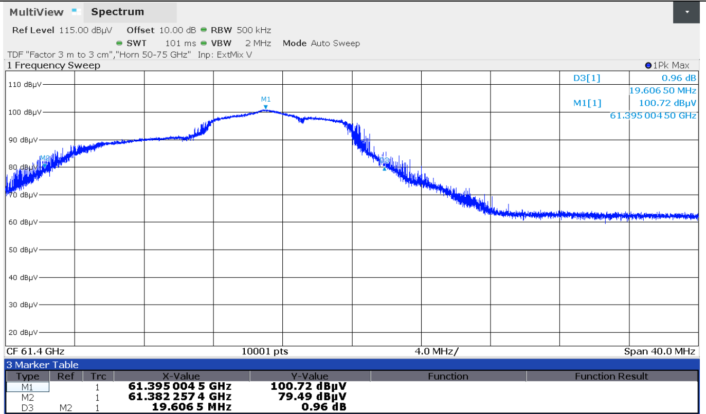
Figure 7.5-3: OBW measurement view high Ch
