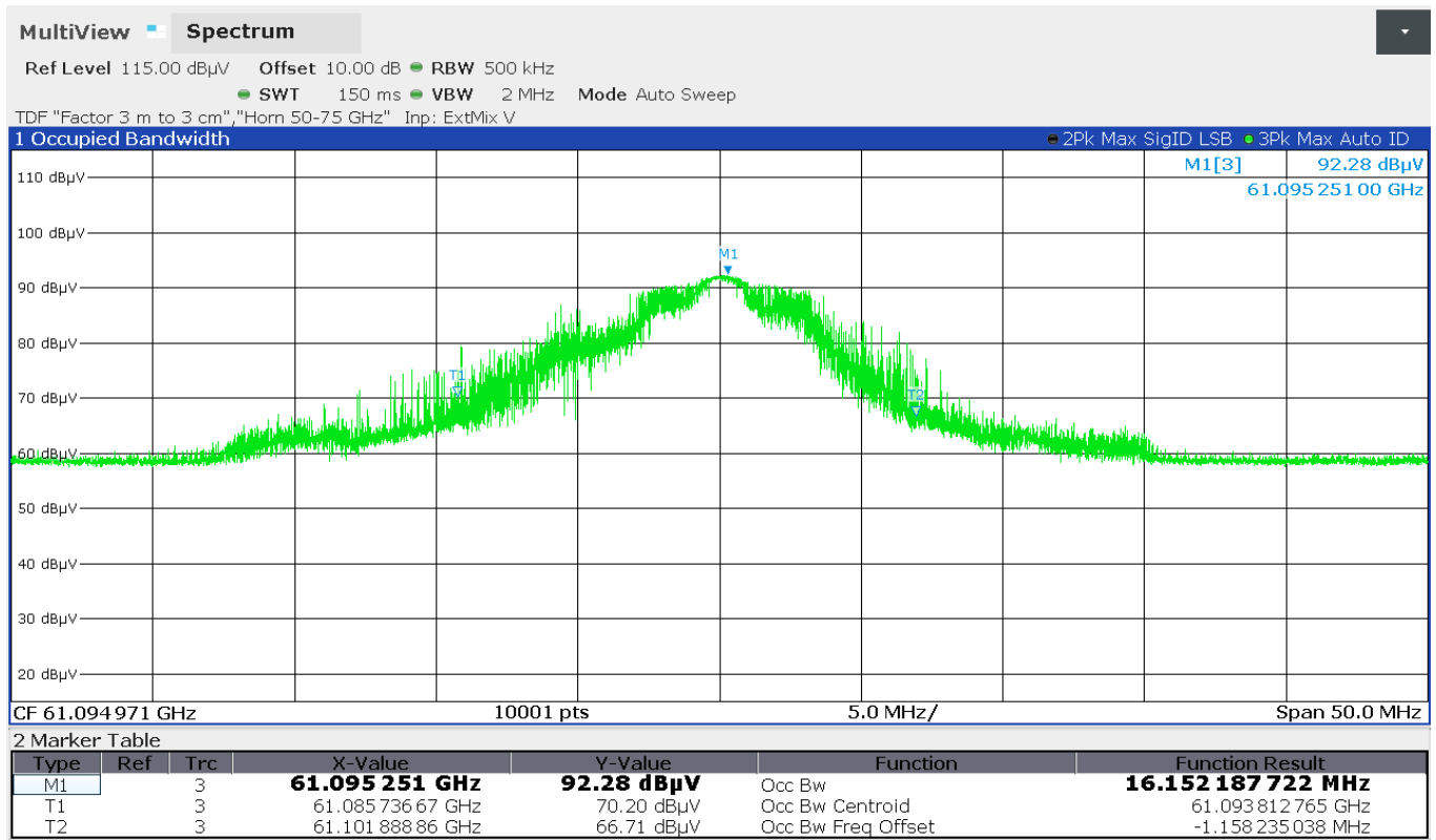
Figure 7.5-4: OBW measurement view Low Ch
