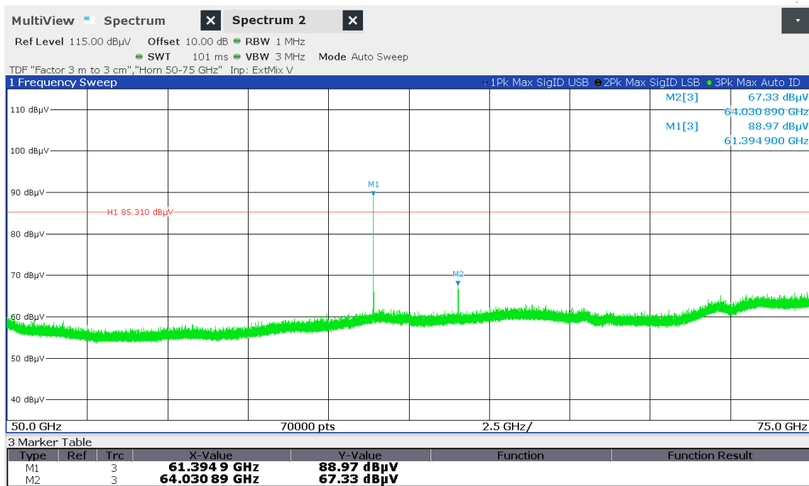
Figure 7.6-5: Radiated spurious emissions 50-75 GHz High Ch
