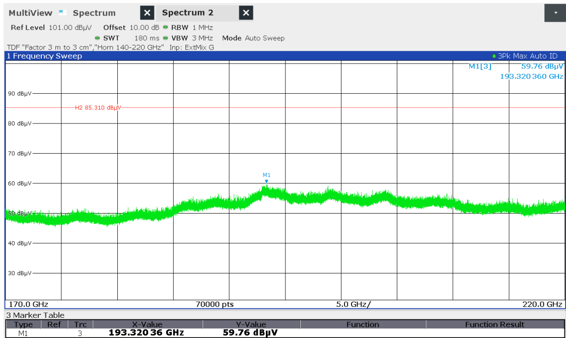
Figure 7.6-9: Radiated spurious emissions 170-220 GHz High Ch
