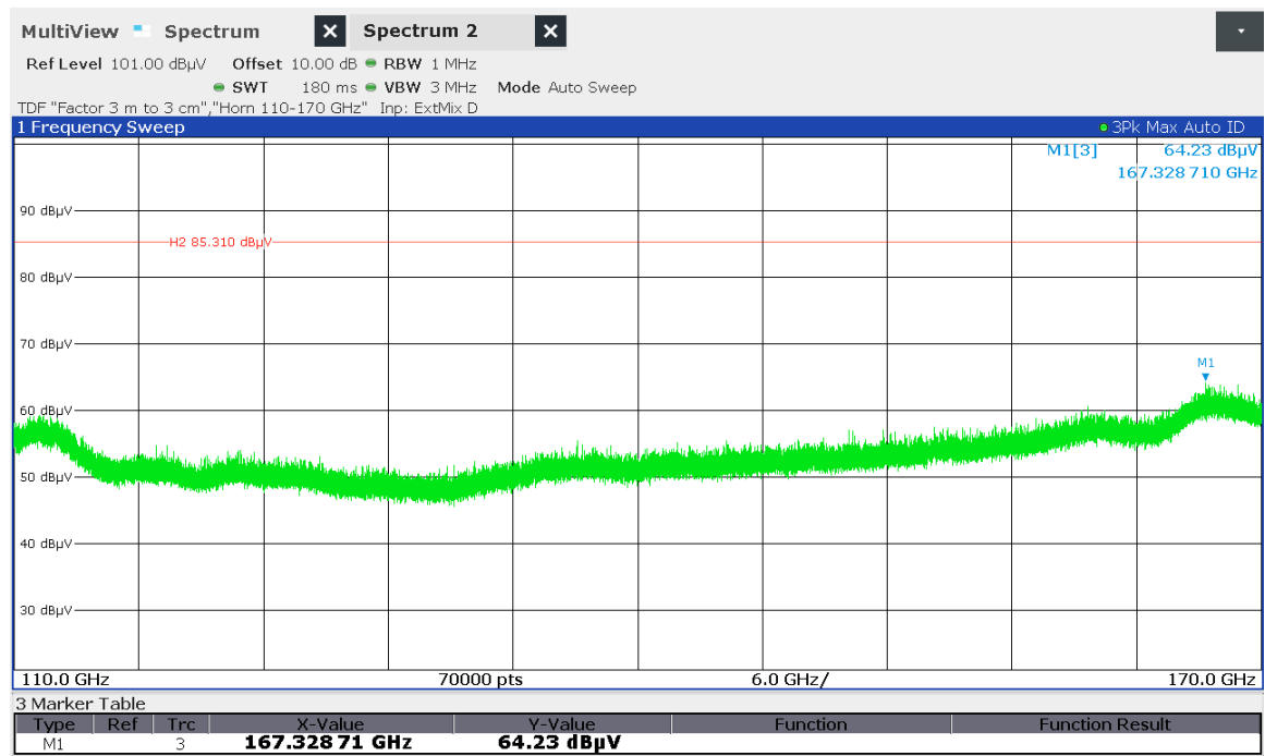
Figure 7.6-18: Radiated spurious emissions 110-170 GHz Low Ch
