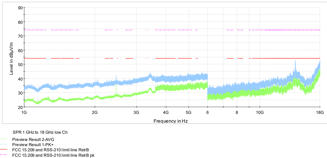
Figure 7.6-11: Radiated spurious emissions above 1-18 GHz Low Ch
