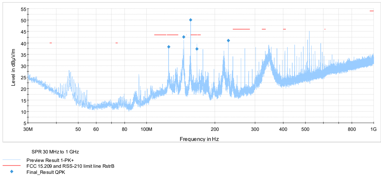
Figure 7.6-1: Radiated spurious emissions below 1000 MHz High Ch
