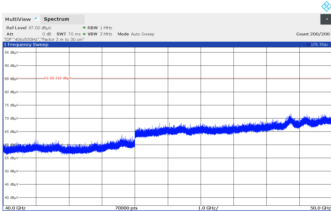
Figure 7.6-4: Radiated spurious emissions 40-50 GHz High Ch
