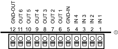
① PCB
