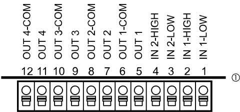
View A
