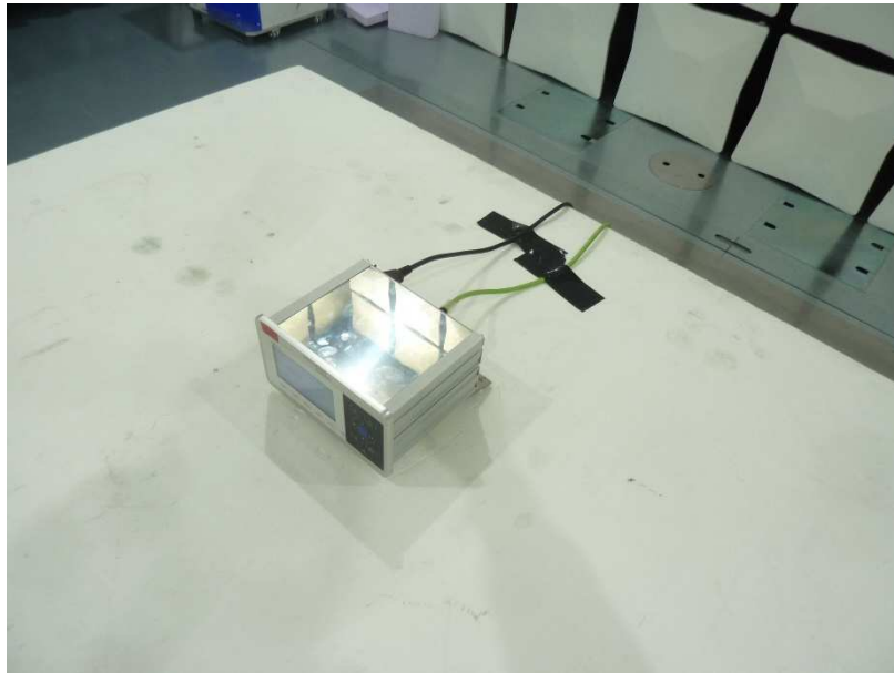
Test setup semi anechoic chamber (normal position)
