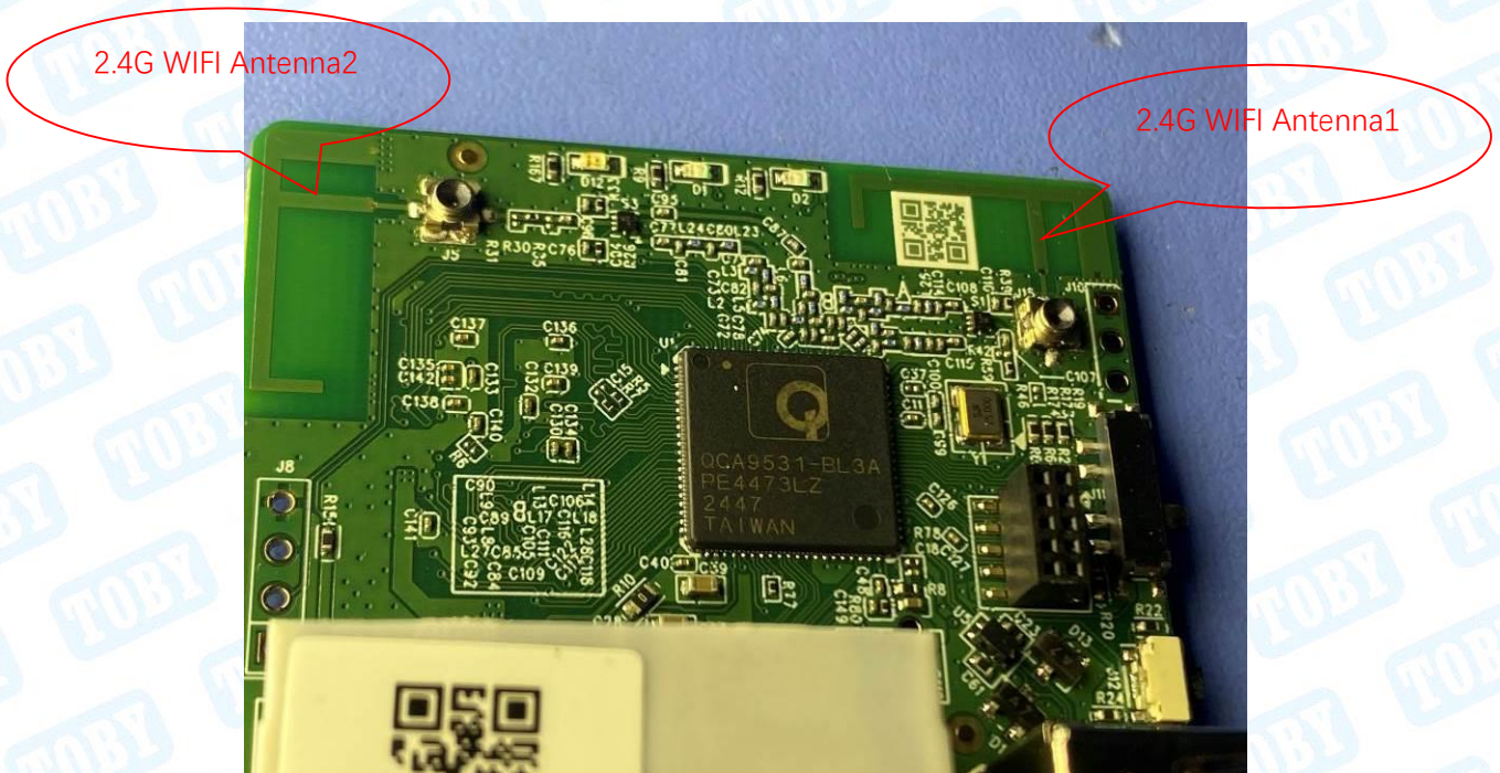
Photo 13 Appearance of PCB
