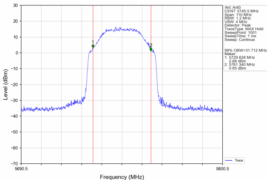
40M_LCH_5745.5MHz_Ant0_NTNV
