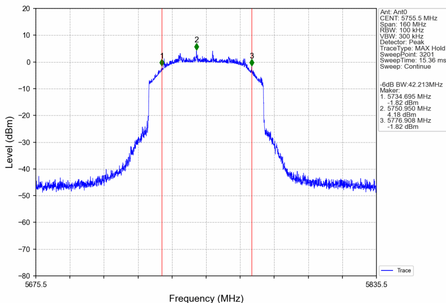
60M_LCH_5755.5MHz_Ant0_NTNV
