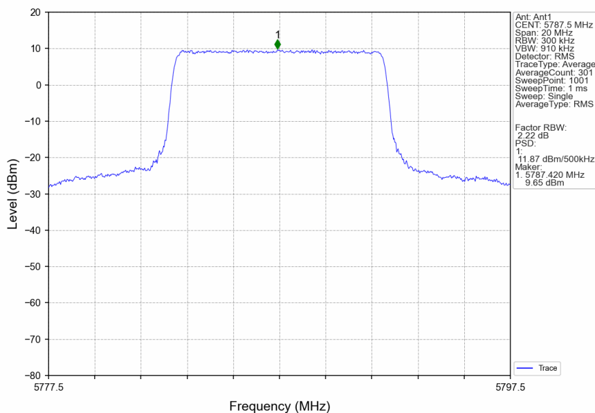
10M_MCH_5787.5MHz_Ant1_NTNV
