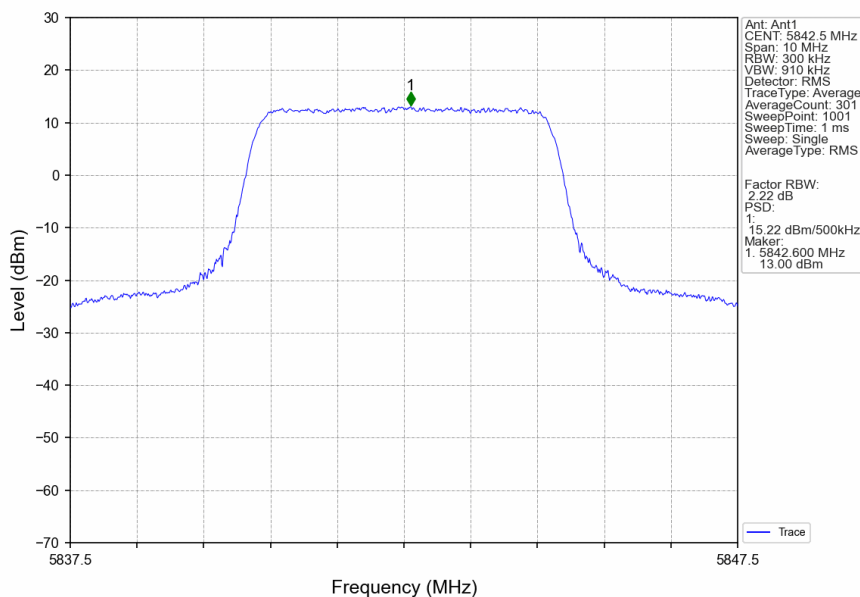
5M_HCH_5842.5MHz_Ant1_NTNV
