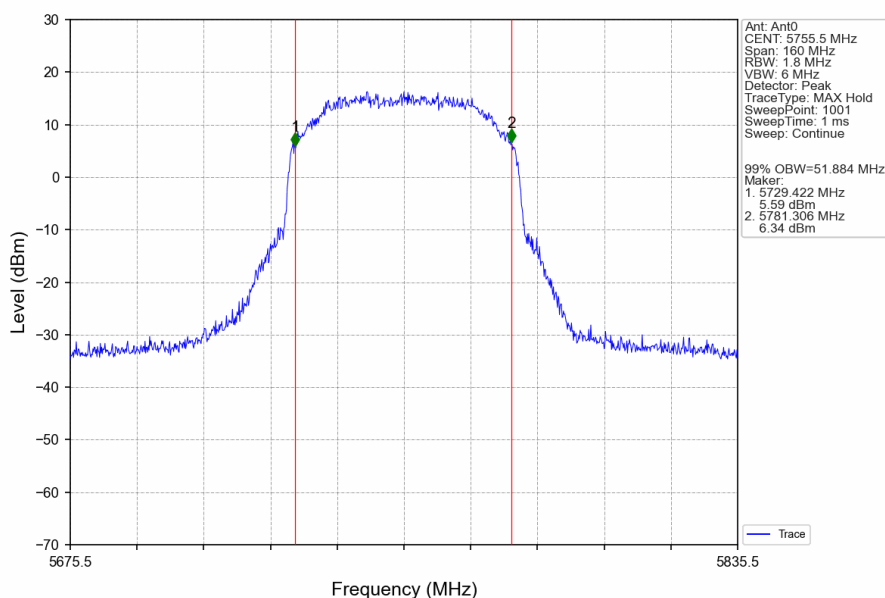
60M_LCH_5755.5MHz_Ant0_NTNV
