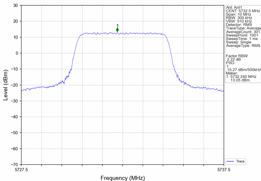
5M_LCH_5732.5MHz_Ant1_NTNV
