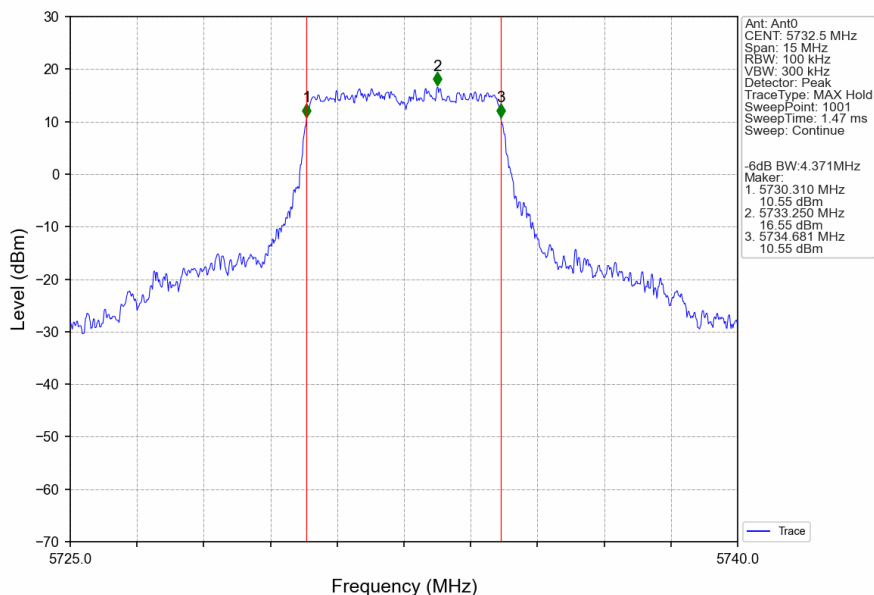
5M_LCH_5732.5MHz_Ant0_NTNV
