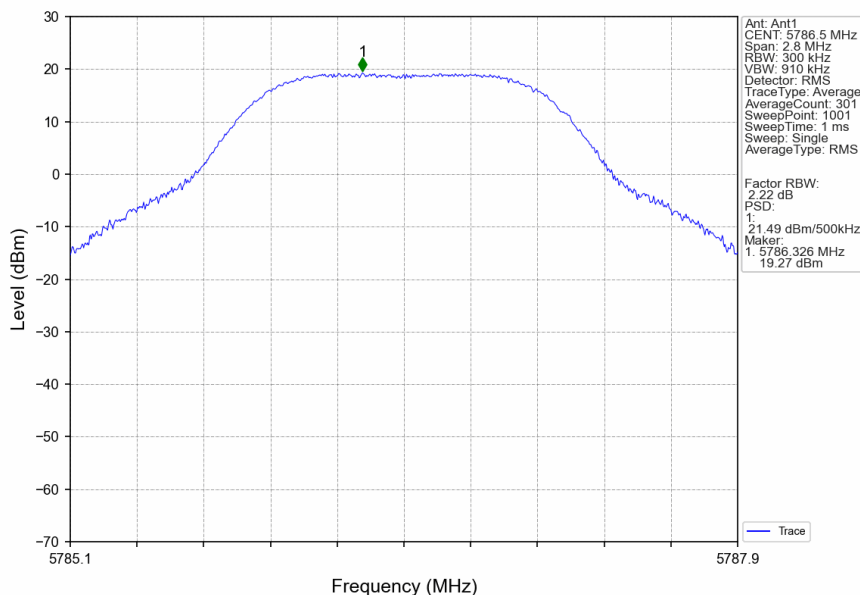
1.4M_MCH_5786.5MHz_Ant1_NTNV
