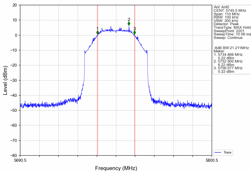
40M_LCH_5745.5MHz_Ant0_NTNV
