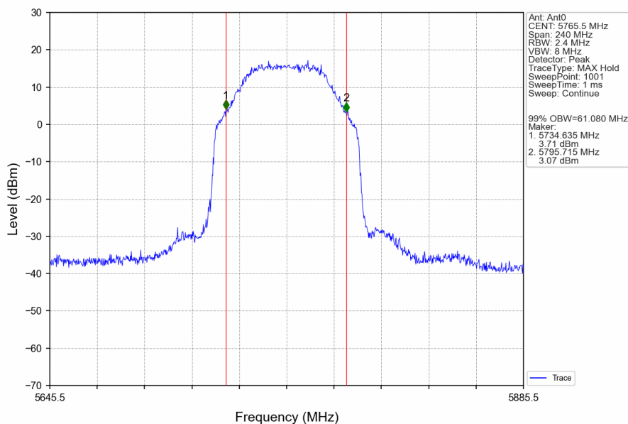
80M_LCH_5765.5MHz_Ant0_NTNV
