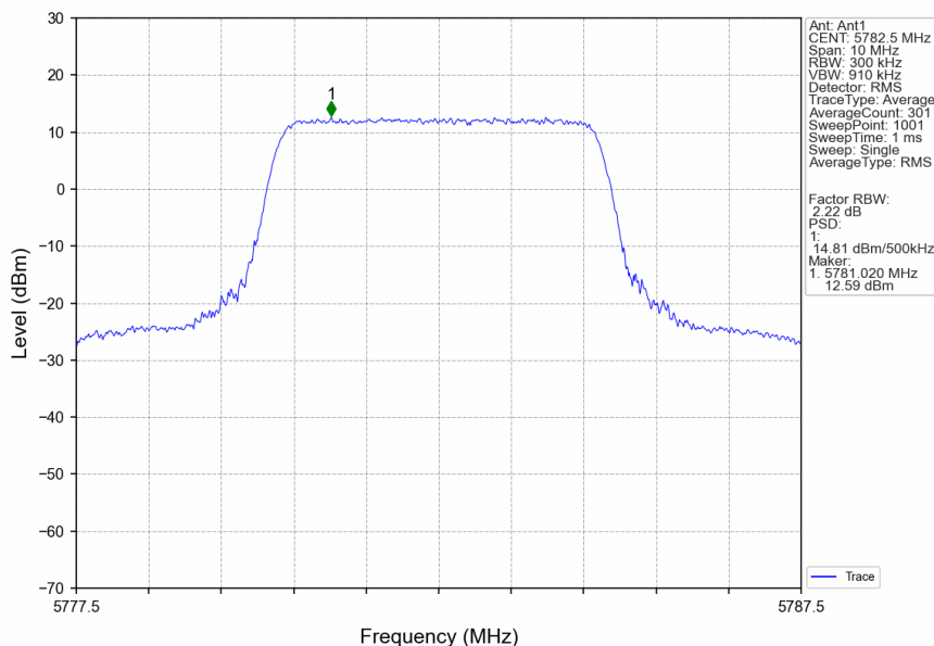
5M_MCH_5782.5MHz_Ant1_NTNV
