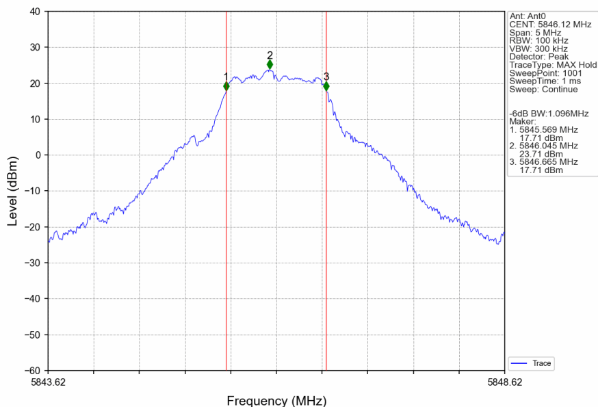
1.4M_HCH_5846.12MHz_Ant0_NTNV
