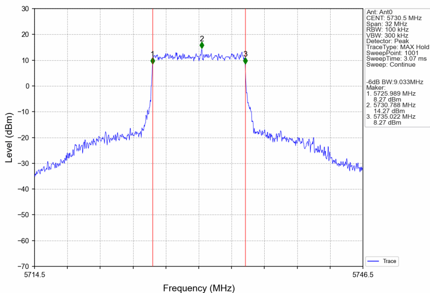
10M_LCH_5730.5MHz_Ant0_NTNV
