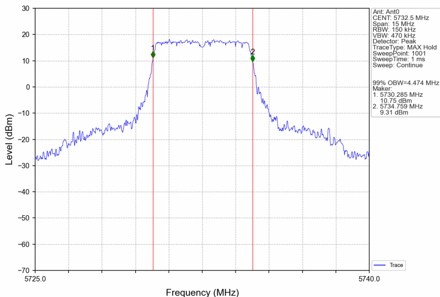
5M_LCH_5732.5MHz_Ant0_NTNV
