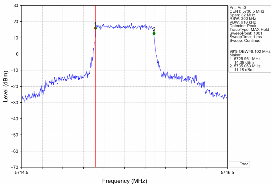
10M_LCH_5730.5MHz_Ant0_NTNV
