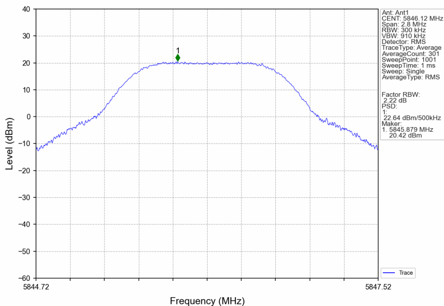
1.4M_HCH_5846.12MHz_Ant1_NTNV
