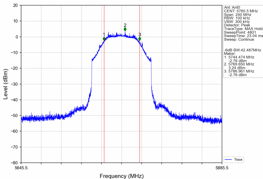
80M_LCH_5765.5MHz_Ant0_NTNV
