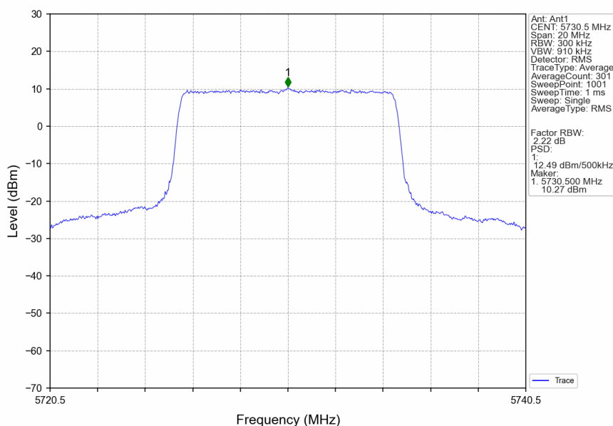
10M_LCH_5730.5MHz_Ant1_NTNV
