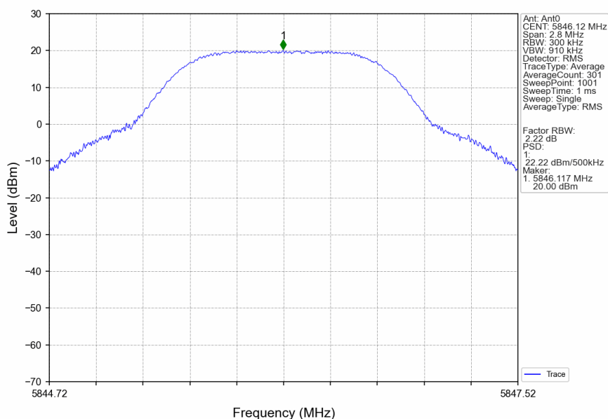
1.4M_HCH_5846.12MHz_Ant0_NTNV
