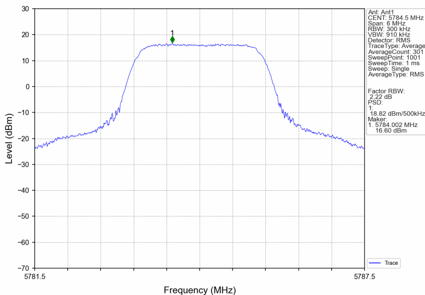
3M_MCH_5784.5MHz_Ant1_NTNV
