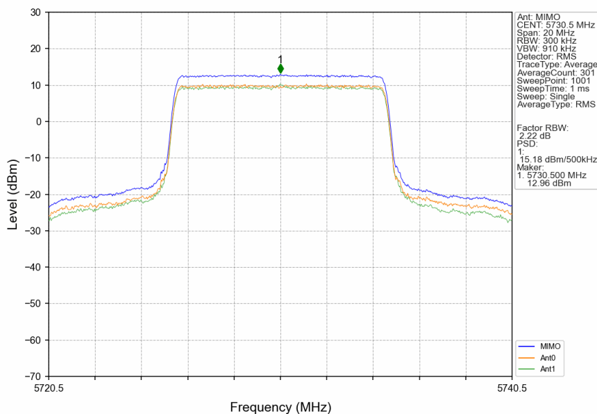
10M_LCH_5730.5MHz_MIMO_NTNV
