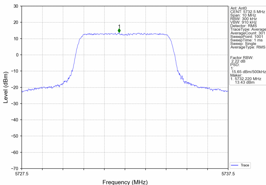
5M_LCH_5732.5MHz_Ant0_NTNV
