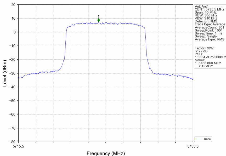
20M_LCH_5735.5MHz_Ant1_NTNV
