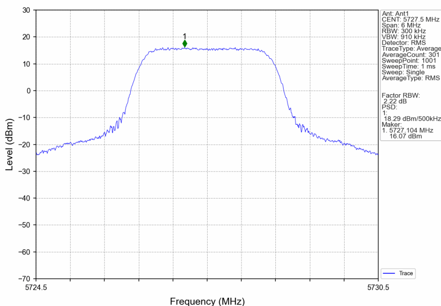
3M_LCH_5727.5MHz_Ant1_NTNV
