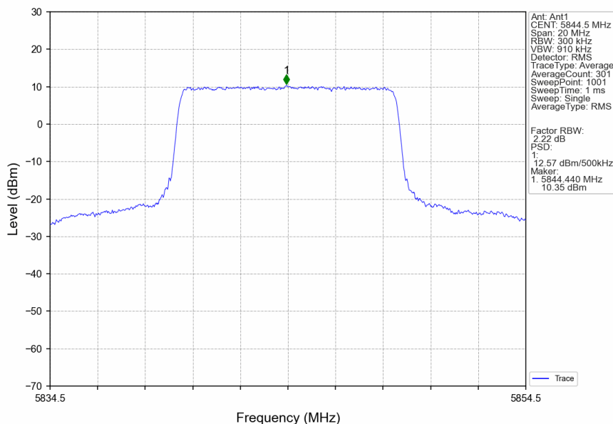
10M_HCH_5844.5MHz_Ant1_NTNV
