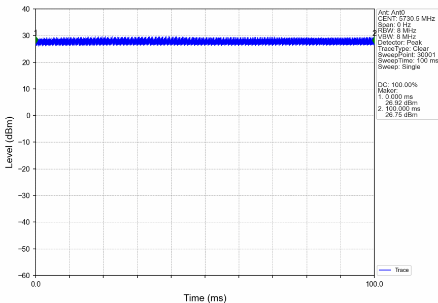
10M_LCH_5730.5MHz_Ant0_NTNV
