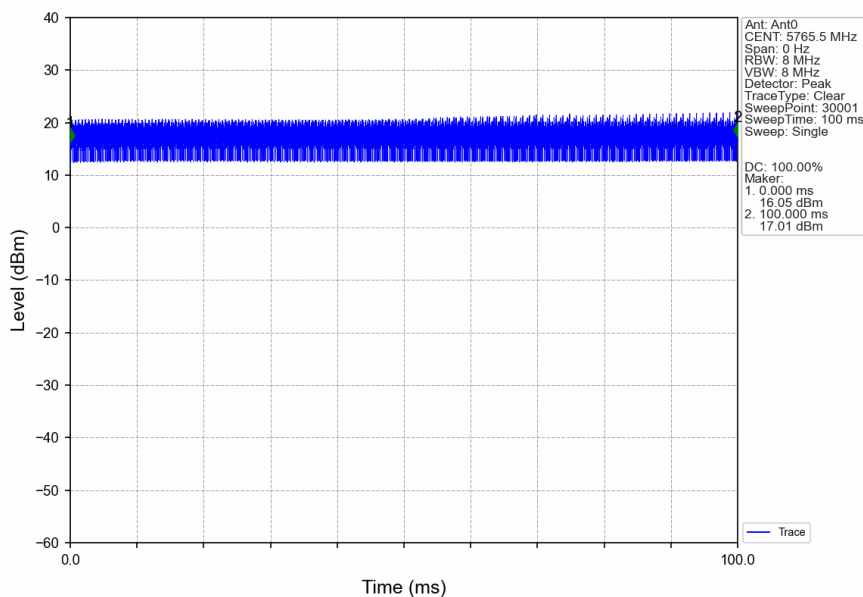
80M_LCH_5765.5MHz_Ant0_NTNV
