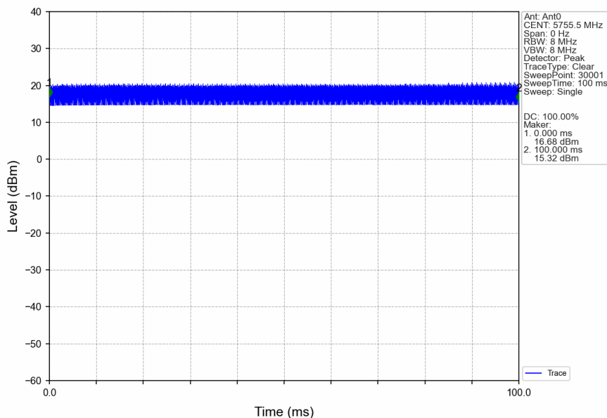
60M_LCH_5755.5MHz_Ant0_NTNV
