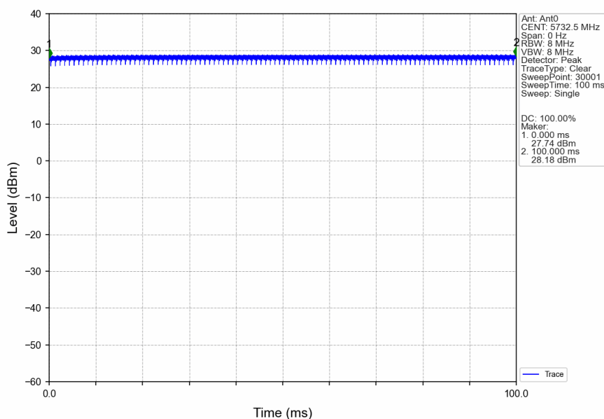
5M_LCH_5732.5MHz_Ant0_NTNV
