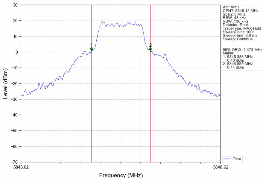
1.4M_HCH_5846.12MHz_Ant0_NTNV
