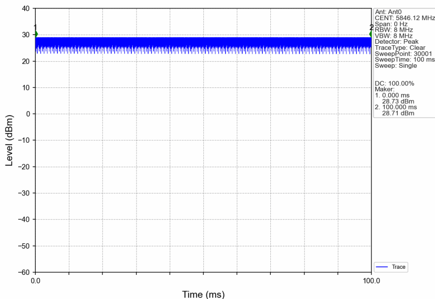
1.4M_HCH_5846.12MHz_Ant0_NTNV
