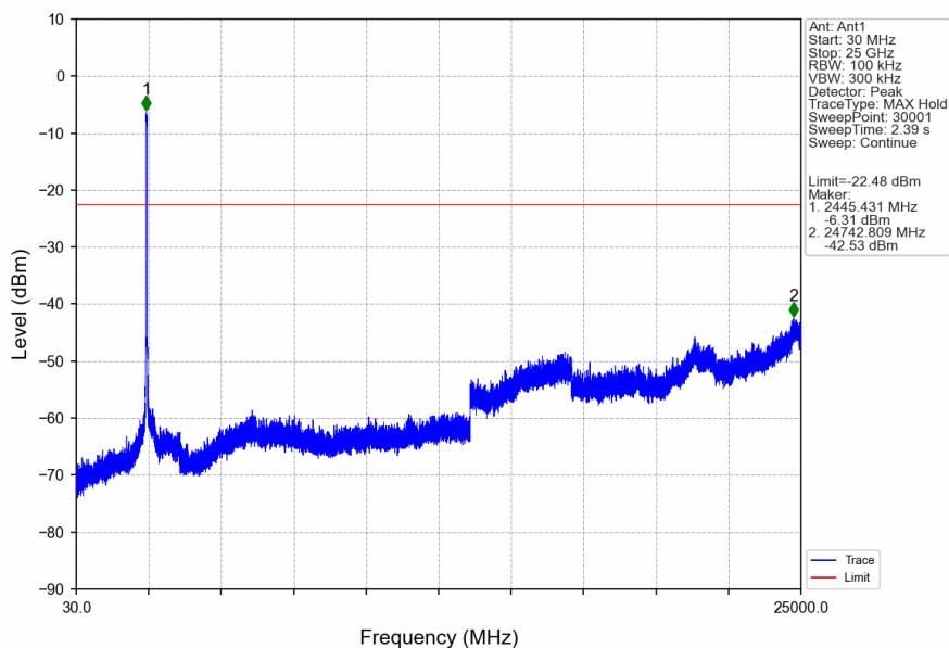
40M_HCH_2452.5MHz_Ant1_NTNV
