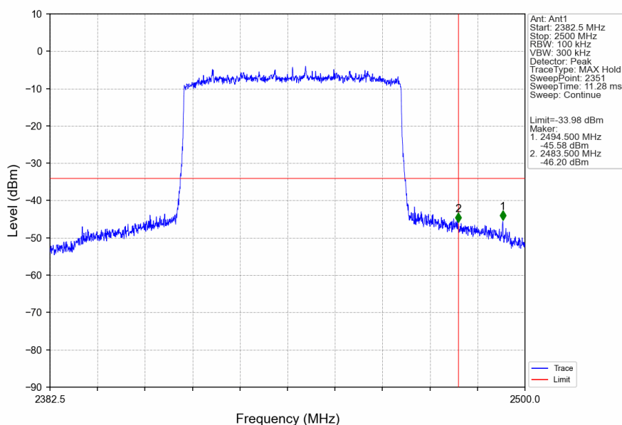
60M_HCH_2442.5MHz_Ant1_NTNV
