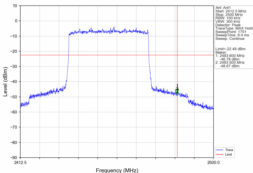
40M_HCH_2452.5MHz_Ant1_NTNV
