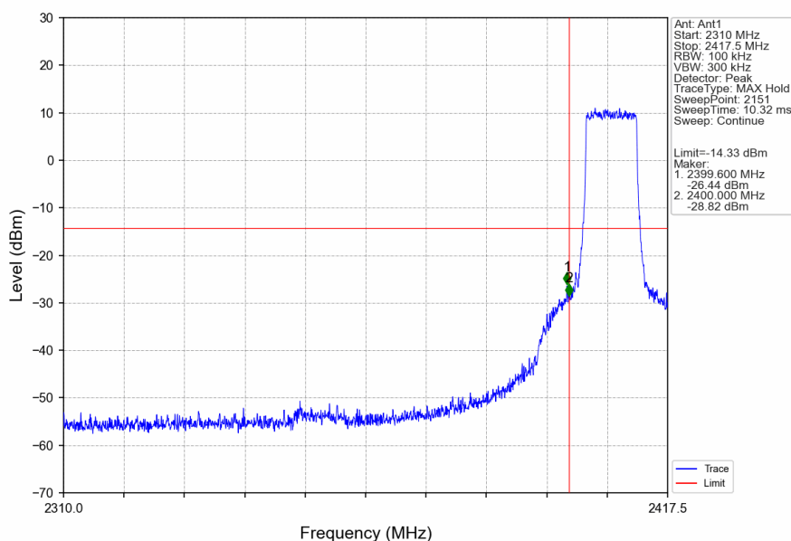
10M_LCH_2407.5MHz_Ant1_NTNV
