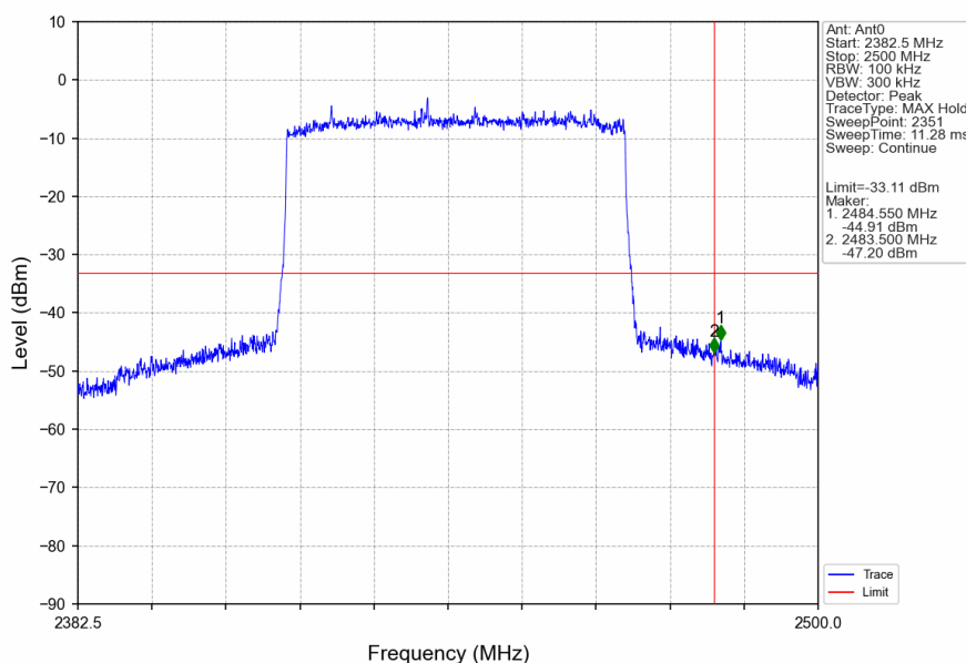
60M_HCH_2442.5MHz_Ant0_NTNV
