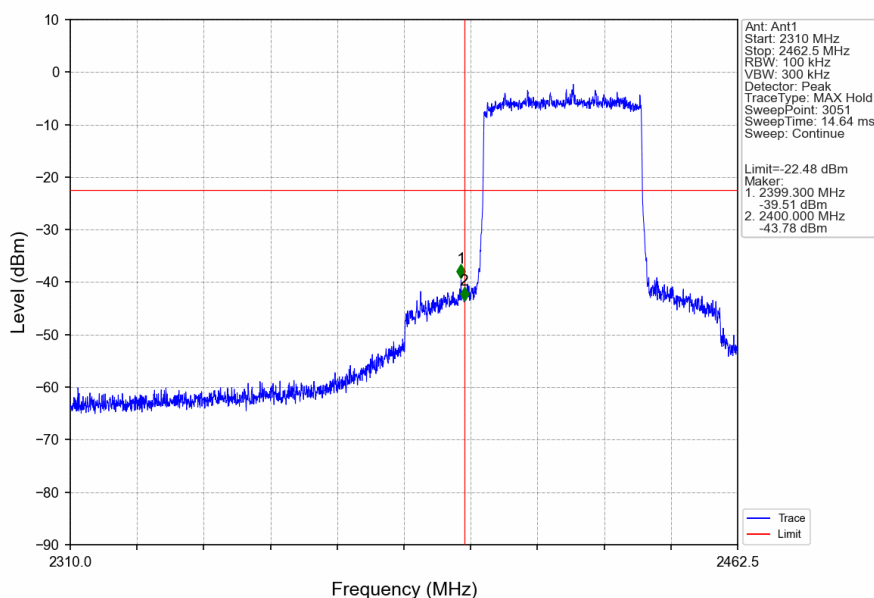
40M_LCH_2422.5MHz_Ant1_NTNV
