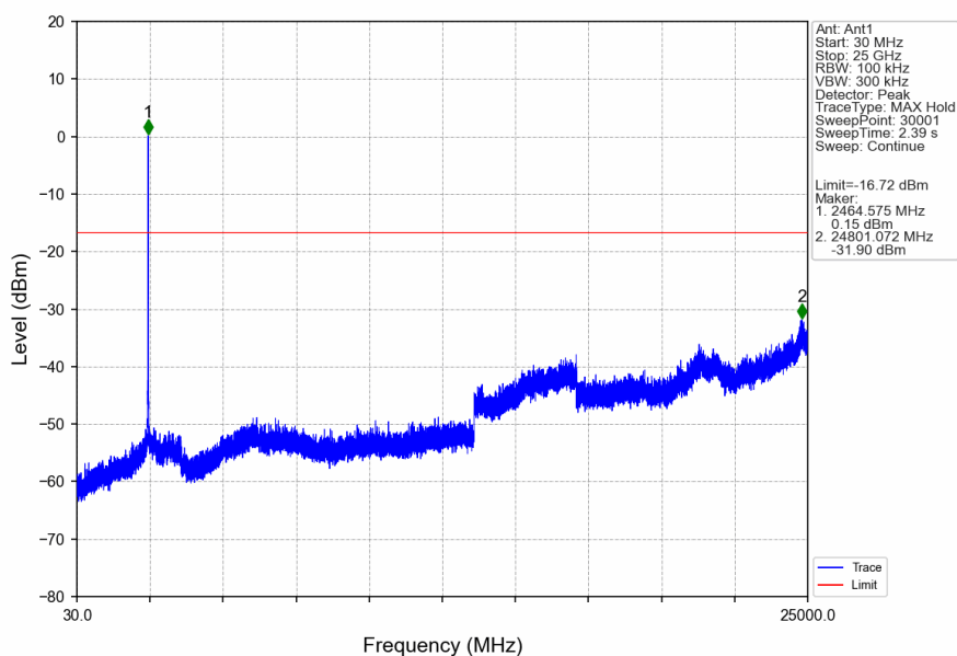
20M_HCH_2462.5MHz_Ant1_NTNV
