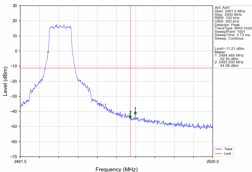
5M_HCH_2469.5MHz_Ant1_NTNV
