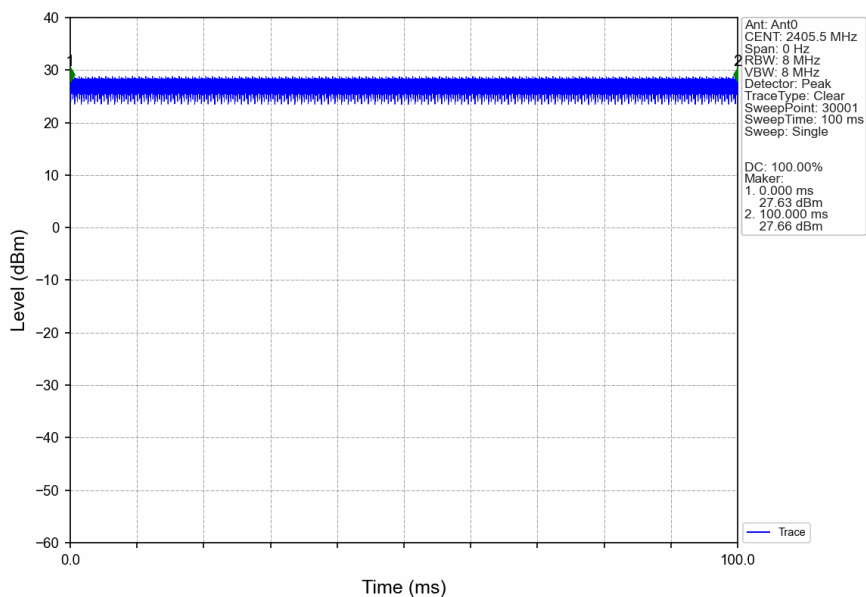
3M_LCH_2405.5MHz_Ant0_NTNV
