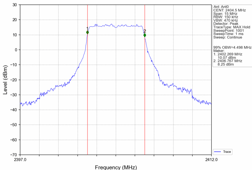
5M_LCH_2404.5MHz_Ant0_NTNV
