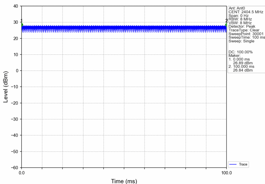
5M_LCH_2404.5MHz_Ant0_NTNV
