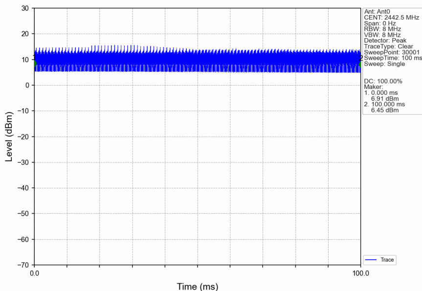
60M_HCH_2442.5MHz_Ant0_NTNV
