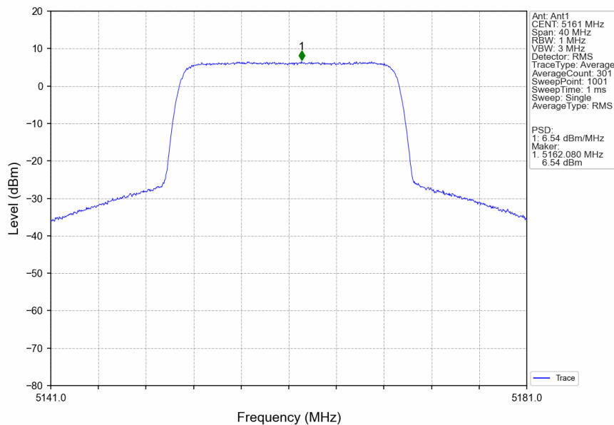
20M_LCH_5161MHz_Ant1_NTNV
