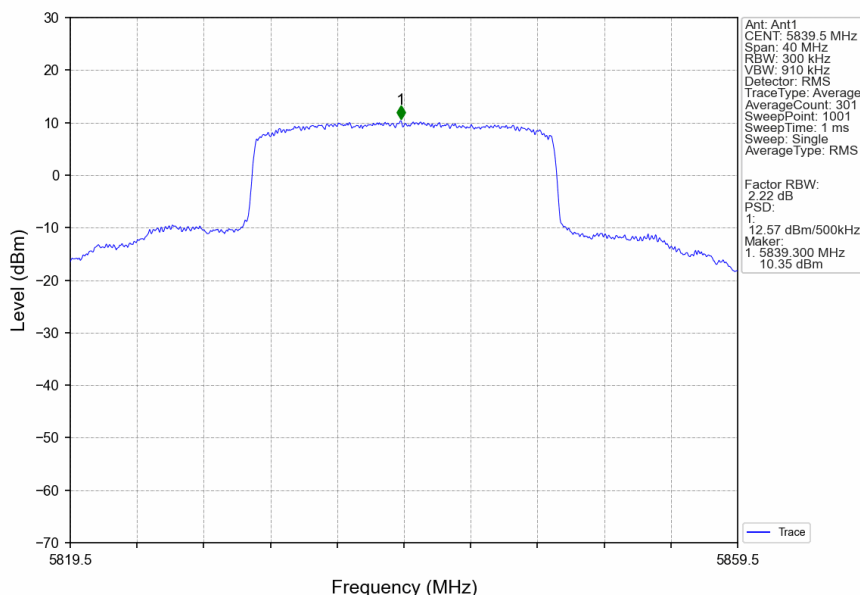
20M_HCH_5839.5MHz_Ant1_NTNV
