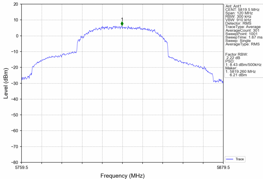
60M_HCH_5819.5MHz_Ant1_NTNV
