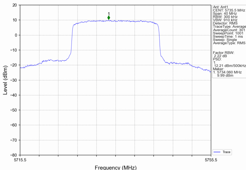
20M_LCH_5735.5MHz_Ant1_NTNV
