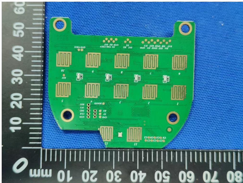
Figure 10. PCB view of unit
