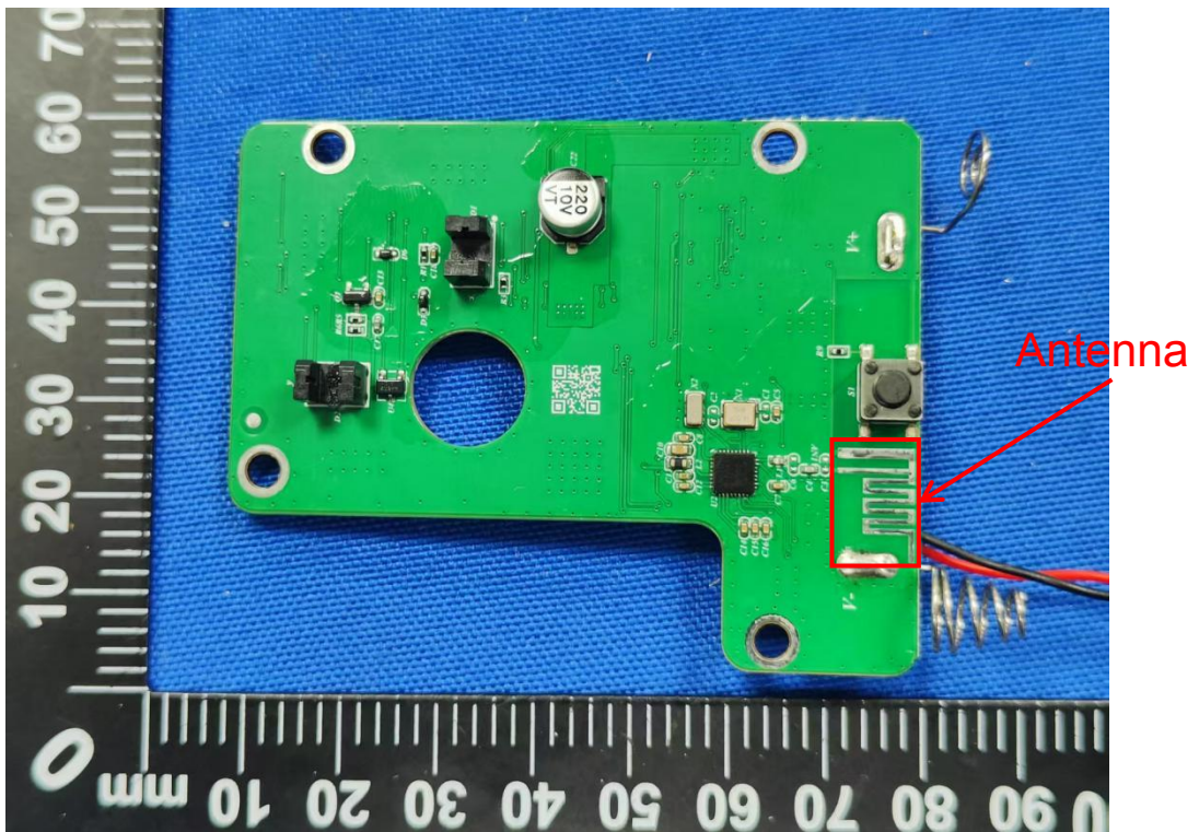
Figure 4. PCB view of unit
