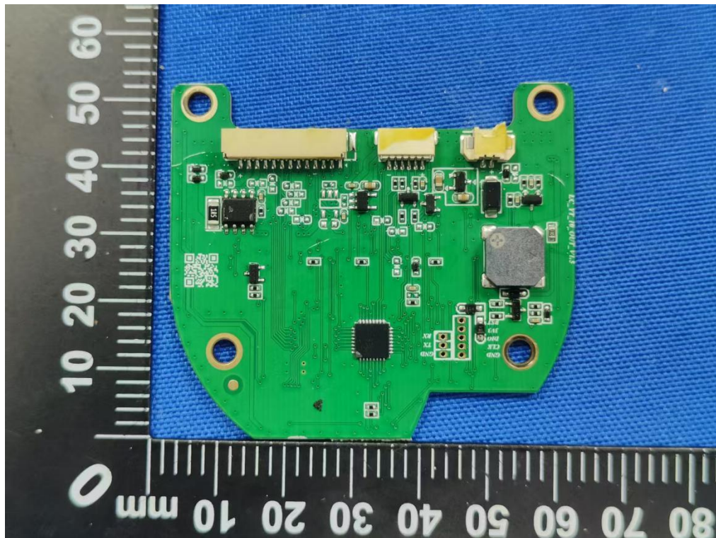
Figure 9. PCB view of unit
