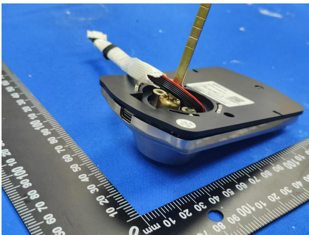
Figure 12. Overall view of unit(Model:WLM13F-SNL)
