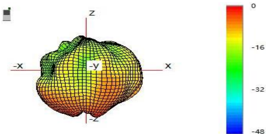
(4) Typical Free Space 3D Radiation Pattern at 6000MHz(unit:dBi):
