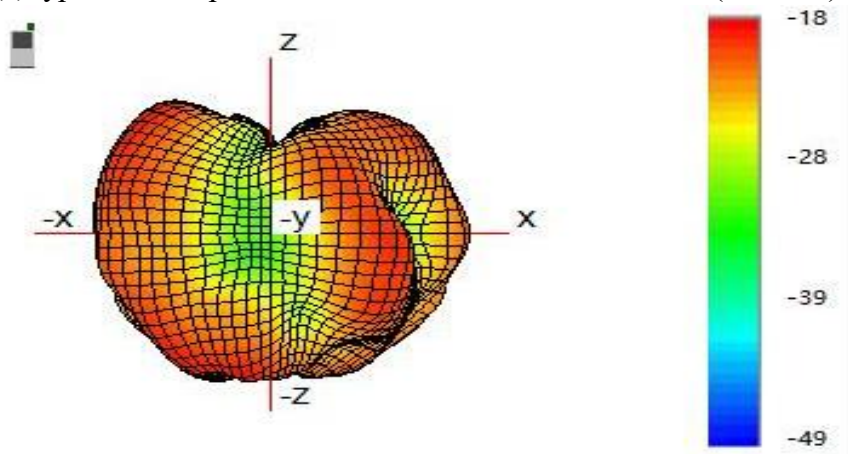
(4)Typical Free Space 3D Radiation Pattern at 2500MHz(unit:dBi):
