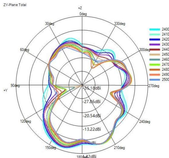
(2) Y-Z Plane(unit:dBi):
