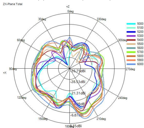
(1) X-Z Plane(unit:dBi):
