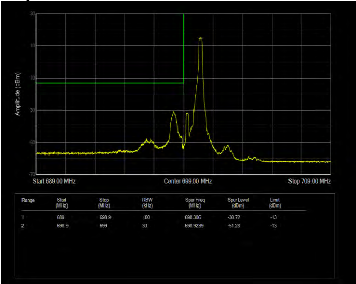
Band12 QPSK BW=1.4MHz Channel=23017 RB Size=6 Position=#0 Extended
