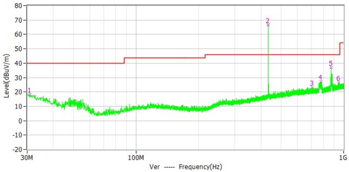
Vertical
