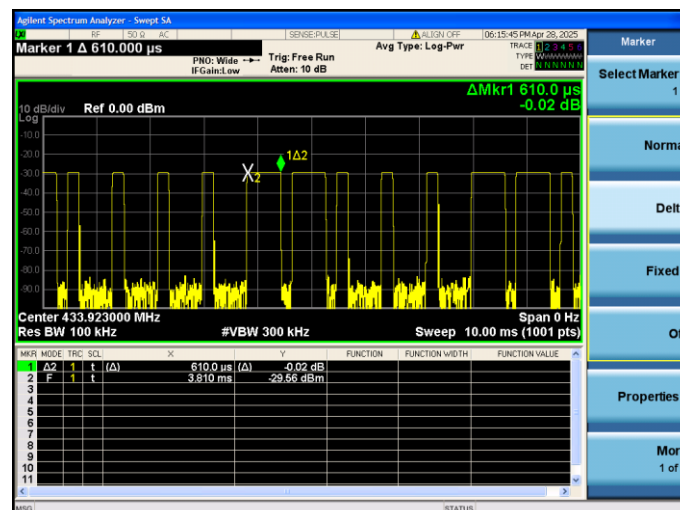
(Time per burst: 0.610ms*8pcs)
