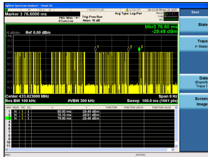
(Transmit cycle 26.60ms)
