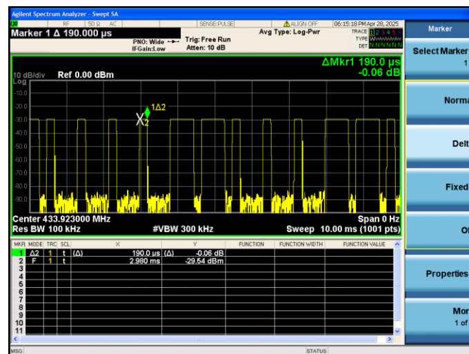
(Time per burst: 0.190ms*17pcs)
