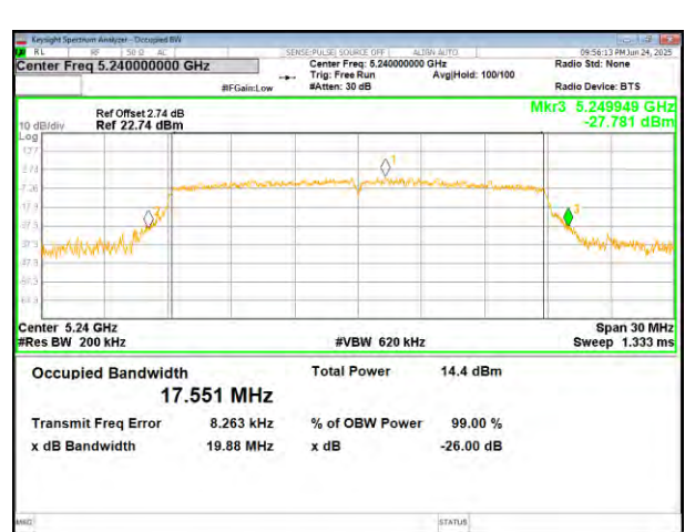
(802.11 n20) plot on channel 48
