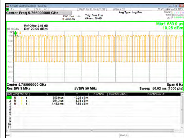
(802.11 ac40) plot
