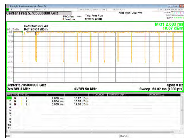
(802.11ac20) plot
