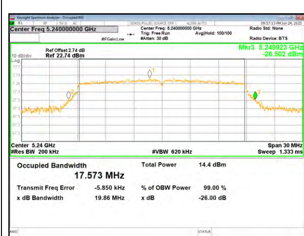
(802.11a) plot on channel 48
