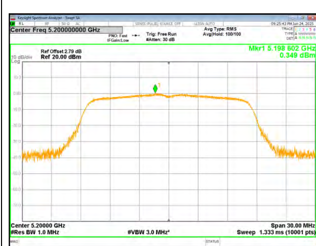
(802.11a) PSD plot on channel 40
