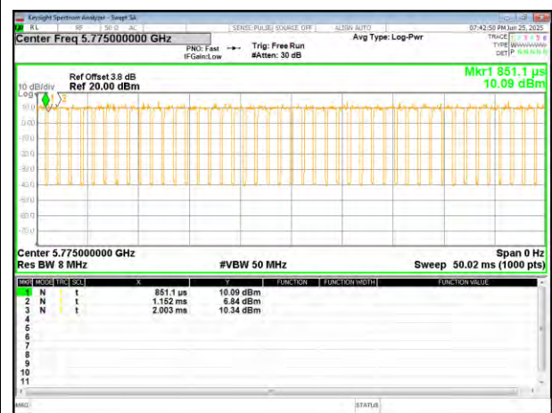
(802.11 ac80) plot
