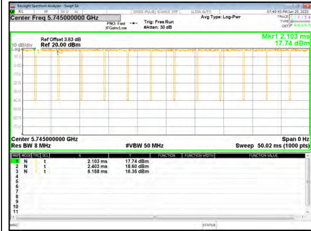
(802.11ac20) plot
