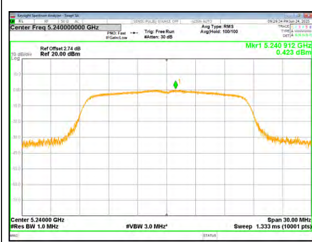
(802.11a) PSD plot on channel 48
