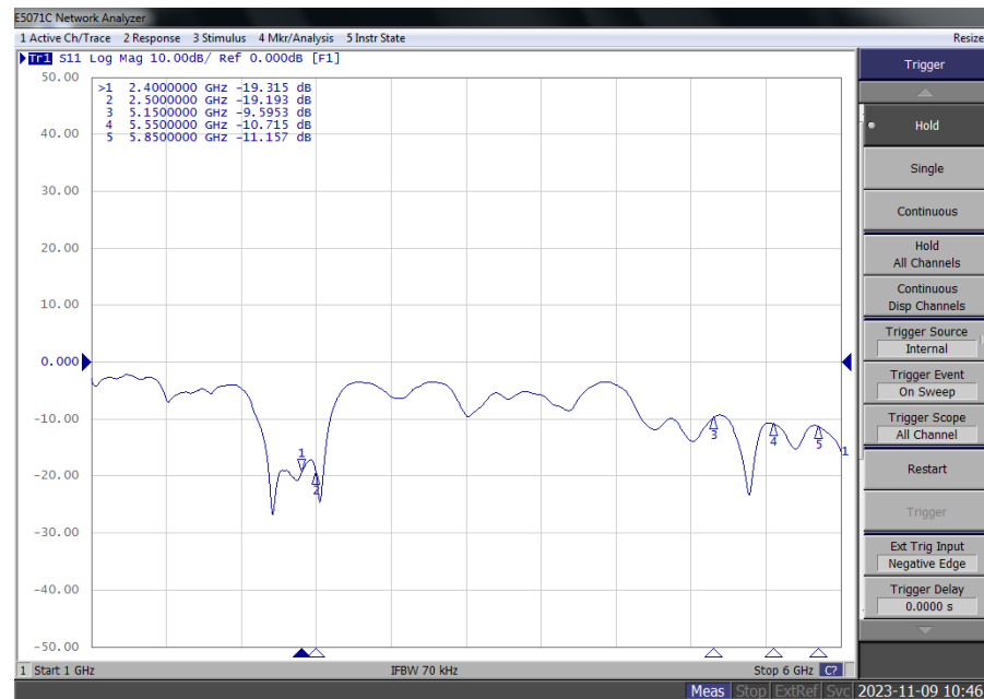
AUX天线S11
