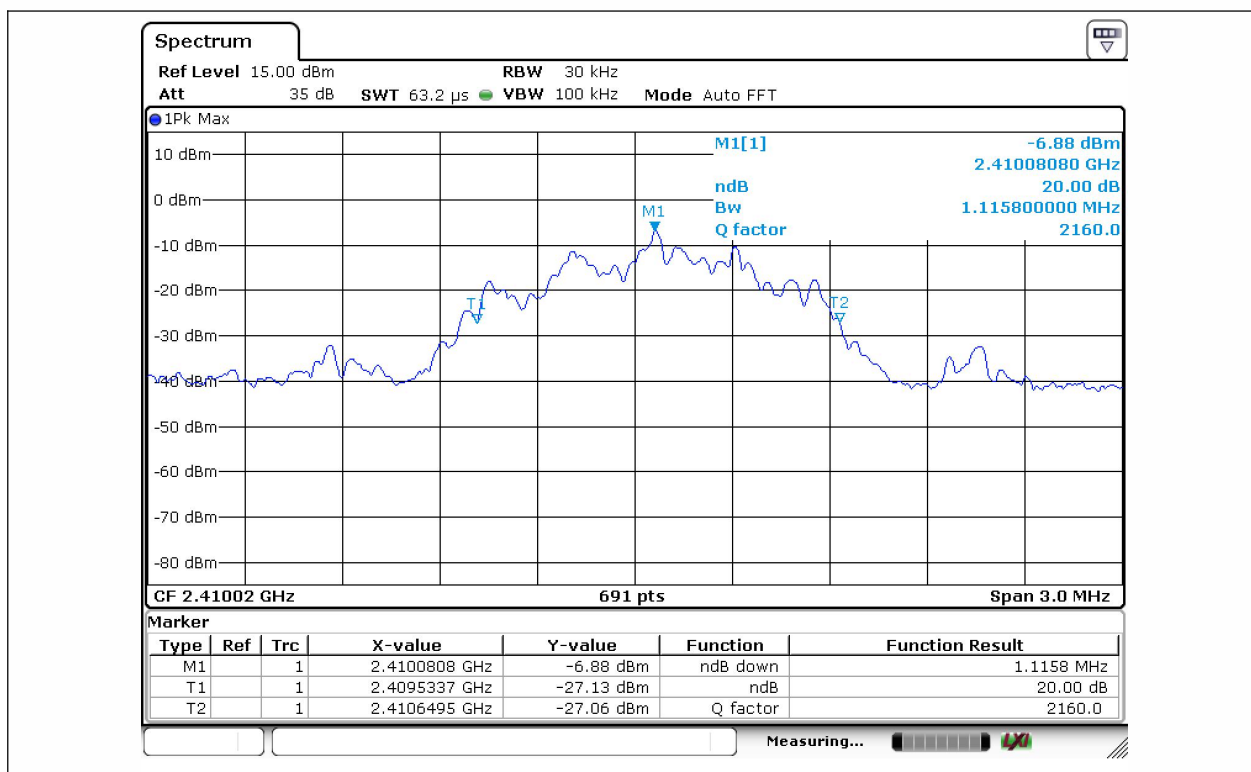
ANT-2410-PASS
