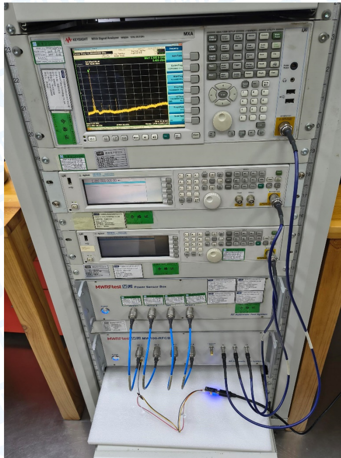
Photo of Setup for RF Conducted
