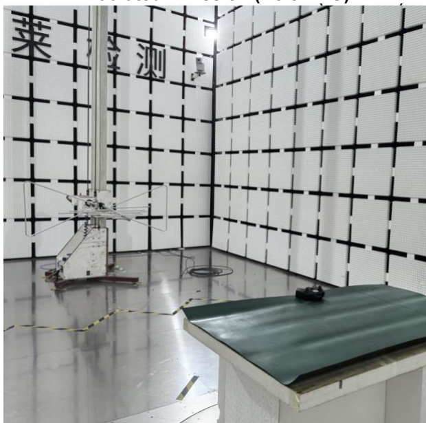
Radiated Emission (Below 1G)
