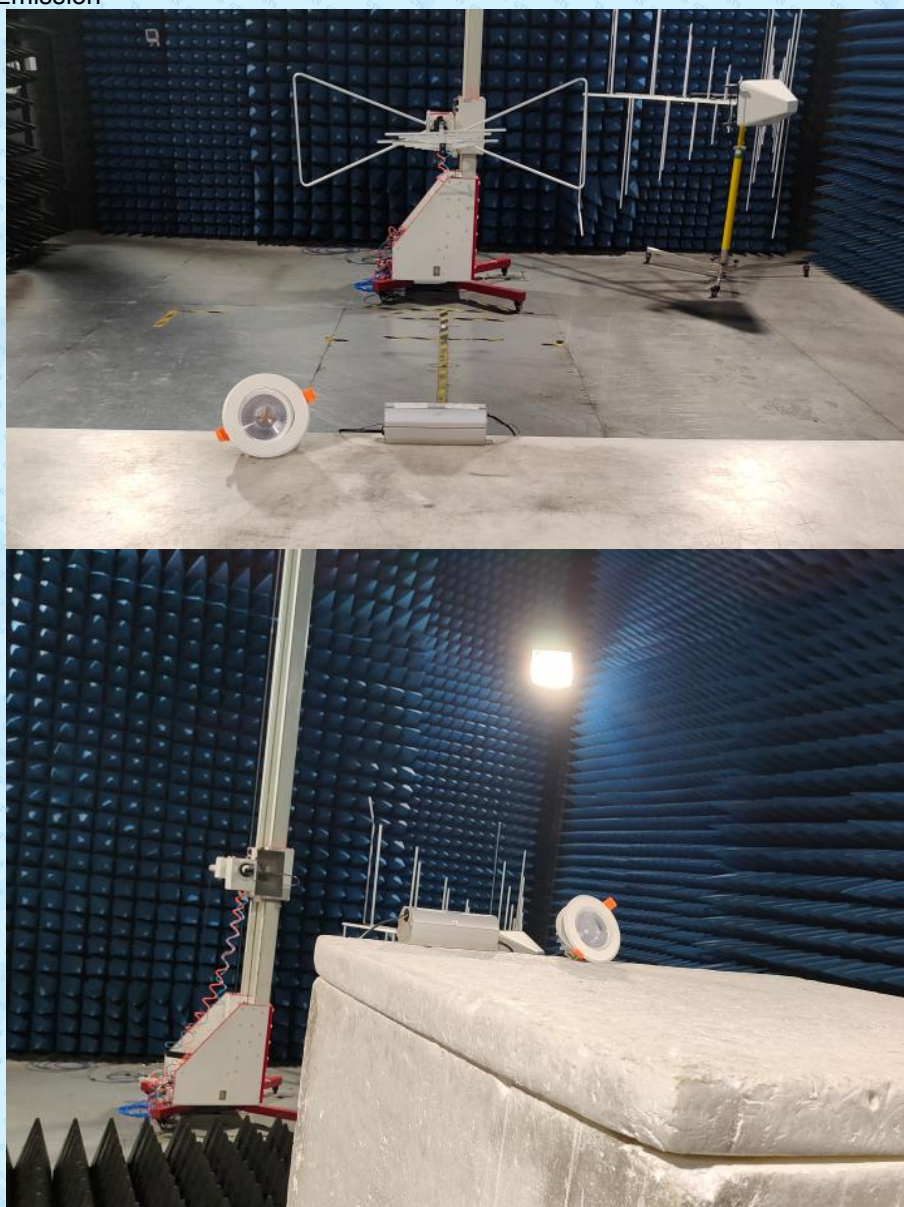
Radiated Emission
