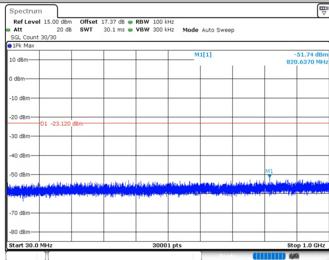
11N20SISO_Ant1_2462_0~Reference
