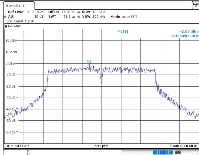
11G_Ant1_2437_0~Reference
