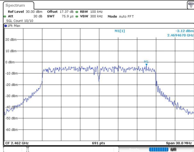
11N20SISO_Ant1_2462_0~Reference
