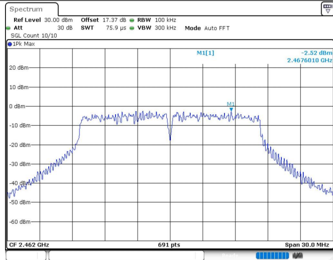
11G_Ant1_2462_0~Reference
