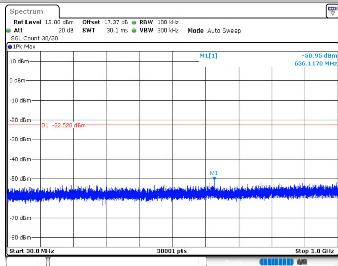
11G_Ant1_2462_0~Reference
