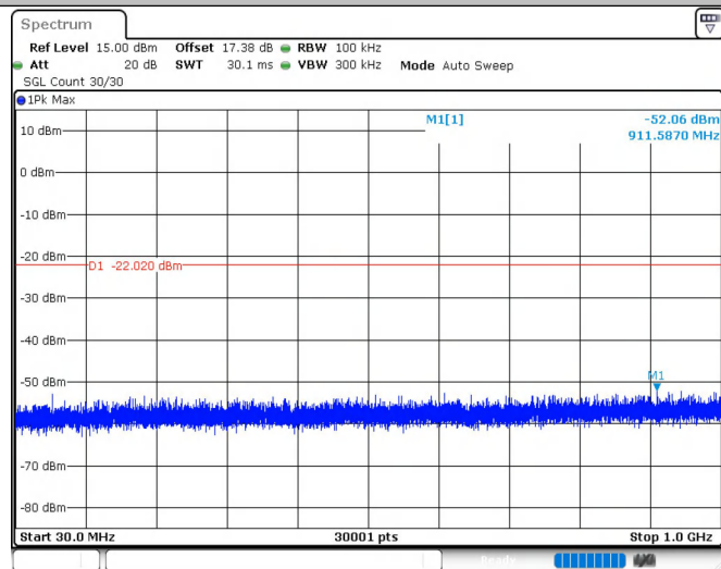
11G_Ant1_2437_0~Reference
