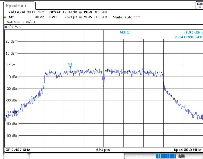
11N20SISO_Ant1_2437_0~Reference
