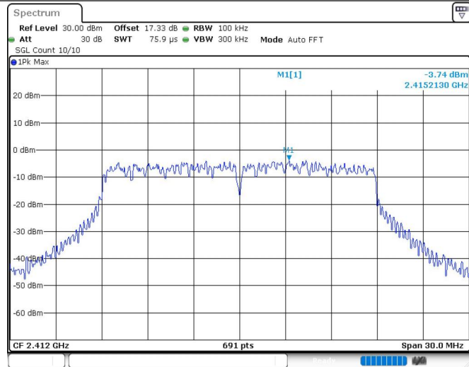
11N20SISO_Ant1_2412_0~Reference
