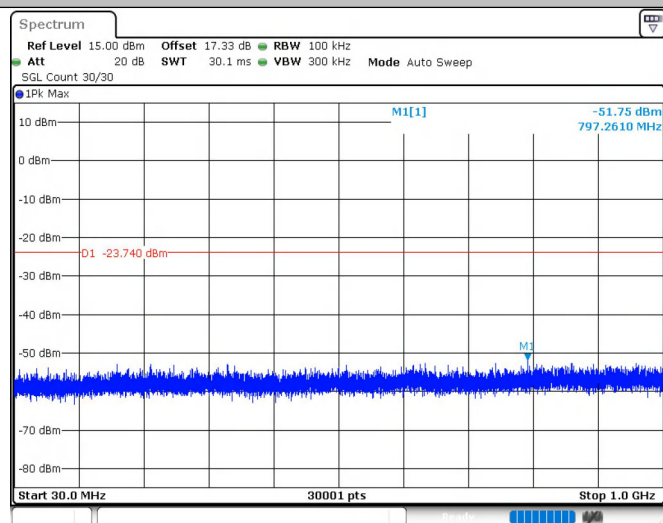
11N20SISO_Ant1_2412_0~Reference
