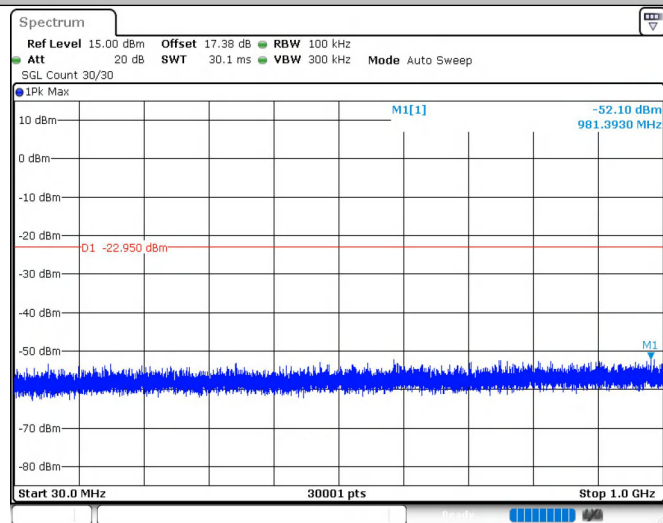
11N20SISO_Ant1_2437_0~Reference
