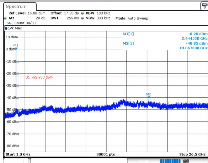
11N20SISO_Ant1_2437_1000~26500
