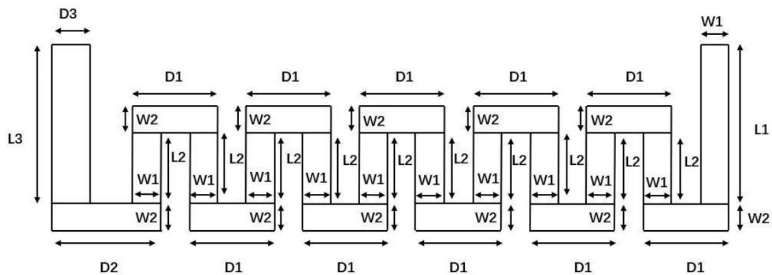
Antenna Dimensions
