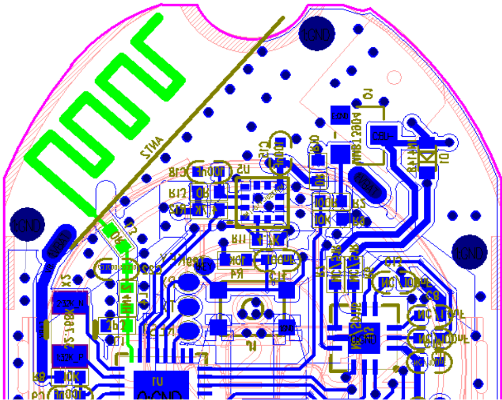
Antenna Photo & Length(mm) 9mm*4mm
