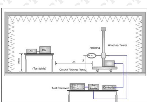
Figure 1. Below 30MHz
