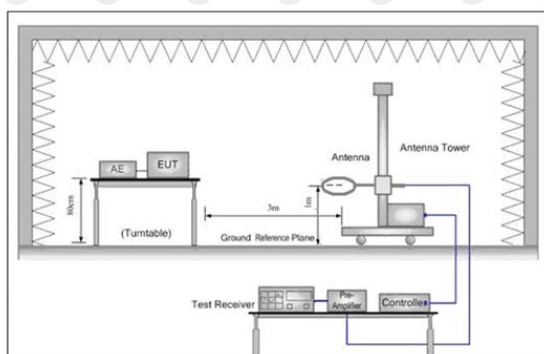
Figure 1. Below 30MHz
